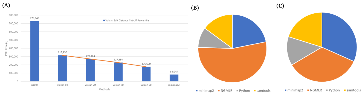
Fig. 3. Comparing runtime for Vulcan, NGMLR and minimap2. CPU time was measured in CPU time for all programs. A: Vulcan achieves an approximately linear acceleration with the increase of the cut-off percentile. With a 90% percentile cut-off, Vulcan only takes about 1/4 of NGMLR’s CPU time. B: The majority of Vulcan’s CPU time is spent in running NGMLR on the subset of reads leading to an improvement of their alignments. C: In 90% percentile cut-off, NGMLR only re-align 10% of the reads, leads to similar time usage as minimap2.
