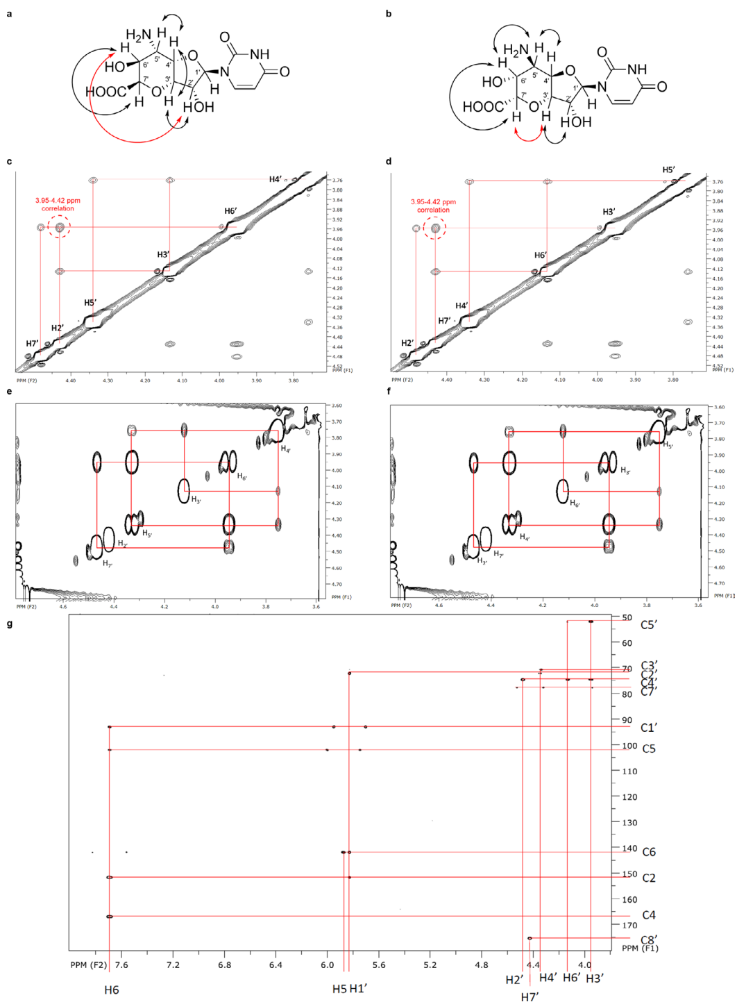
Supplementary Figure 17. Stereochemical revision of AHOA. a and b . Original ( a ) and revised ( b ) structure of AHOA with NOESY correlations shown in double-headed arrows (3.95–4.42 ppm correlation shown in red). c and d . ^1\text{H} - ^1\text{H} NOESY spectrum of AHOA with the original ( c ) and revised ( d ) signal assignment. e and f . ^1\text{H} - ^1\text{H} COSY spectrum of AHOA with original ( e ) and revised ( f ) signal assignments. g . HMBC spectrum of AHOA with the revised signal assignments.
