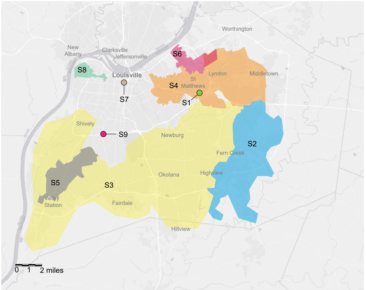
Supplementary Figure 1: Wastewater sampling catchments in Louisville (Kentucky), Sites 1 and 7 represent collection sites of hospitals and Site 9 is a sewer district facility.
