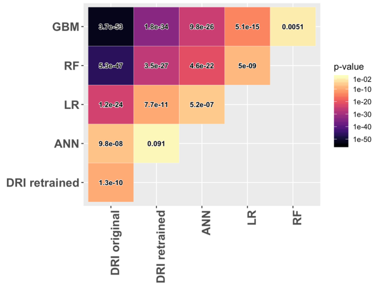
Figure S1: Significance of difference test between the ROC from different models. Testing was performed using de Long method.
