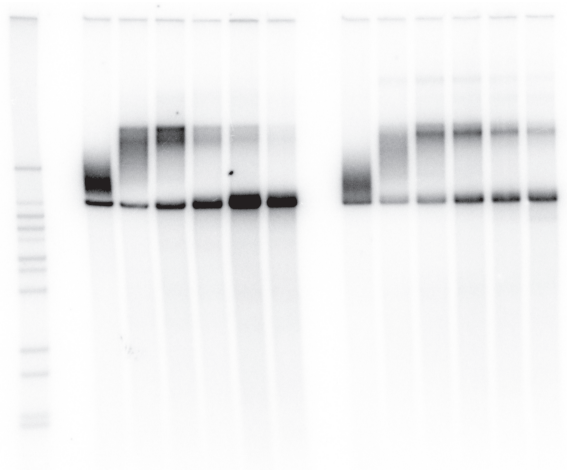
Figure 3 - HO, native
