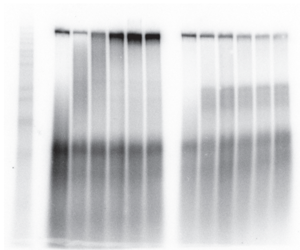
Figure 3 - CD, denaturing
