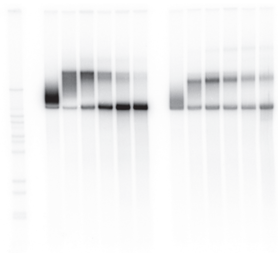
Figure 3 - CD, native
