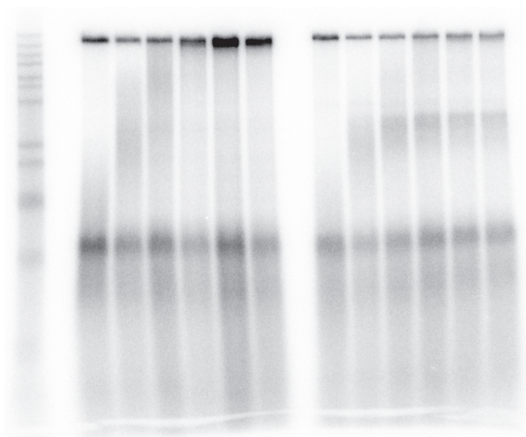
Figure 3 - HO, denaturing
