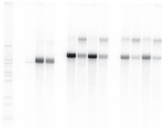
Figure 4D - native
