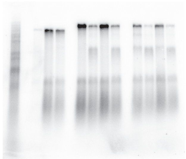
Figure 4D - denaturing
