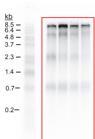
Figure 6D - denaturing
