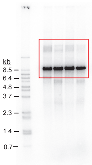
Figure 6D - native
