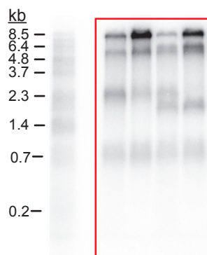
Figure 6C
