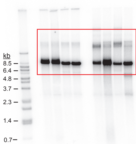
Figure 6A - native
