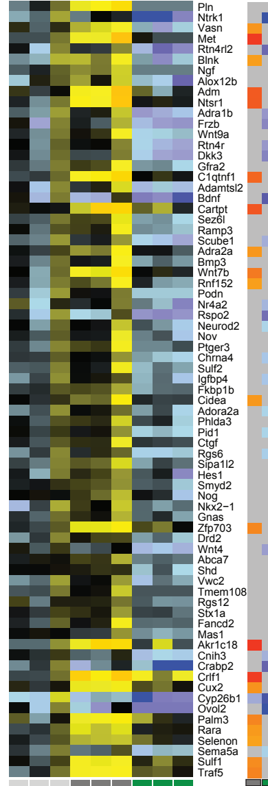
GO:0009966 Regulation of signal transduction
