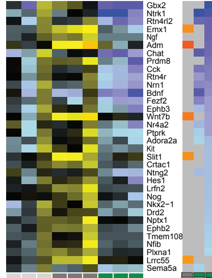
GO:0010975 Reg. of neuron projections development
