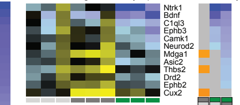
GO:0040012 Regulation of locomotion
