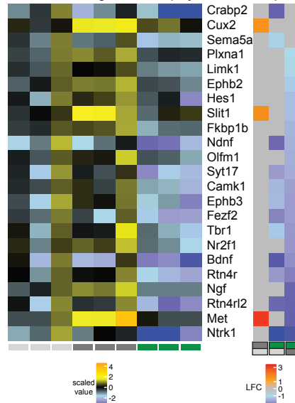
GO:0010975 Reg. of neuron projections development
