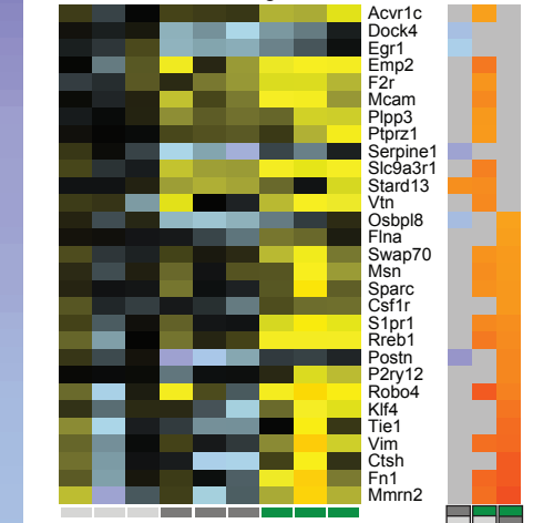
GO:0040012 Regulation of locomotion
