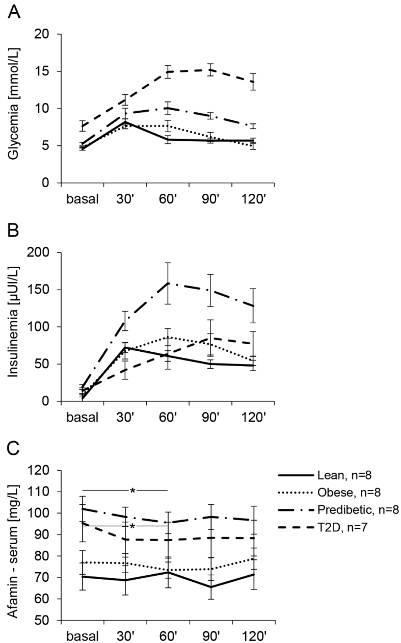
Supplementary Figure 1. (A) Glycemia, (B) insulinemia and (C) serum afamin concentrations during oGTT. Data are presented as mean \pm SEM. * p < 0.05 ; One-way repeated measures ANOVA (Turkey multiple comparison test).
