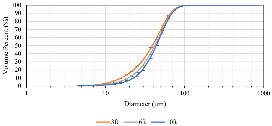
Airofog Cumulative Distribution DI
