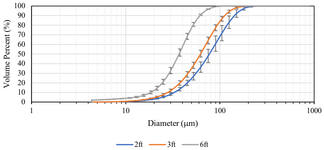
PX200 HH ES On Cumulative Distribution Tap
