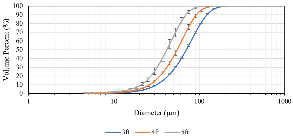
R40 Cumulative Distribution Tap
