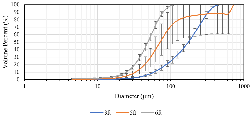
Garden sprayer Cumulative Distribution Tap
