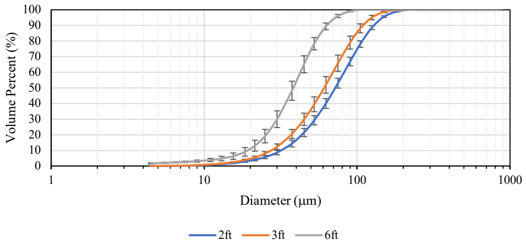
PX200 HH ES Off Cumulative Distribution Tap
