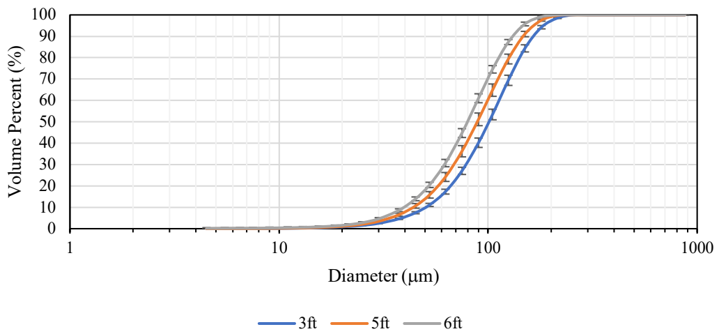
EM360 Cumulative Distribution DI
