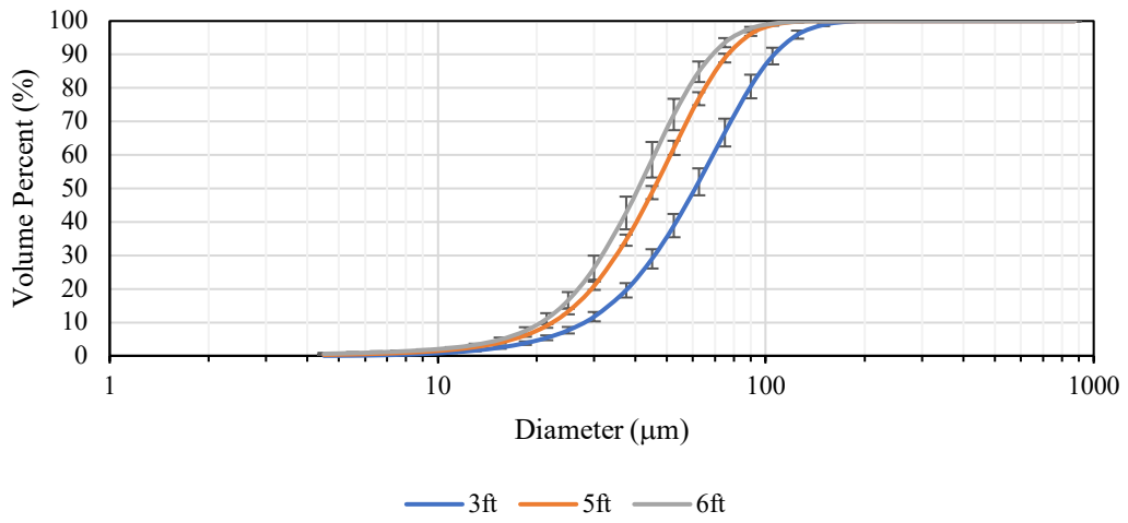
PX 300 Red nozzle Cumulative Distribution Tap
