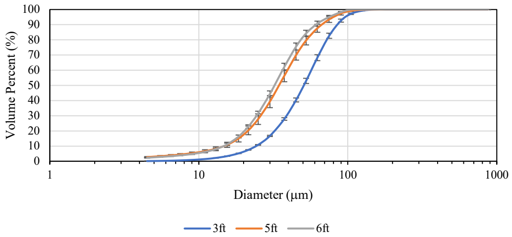
PX 300 green nozzle Cumulative Distribution Tap
