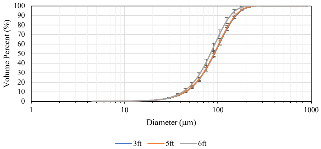
EM360 Cumulative Distribution Tap
