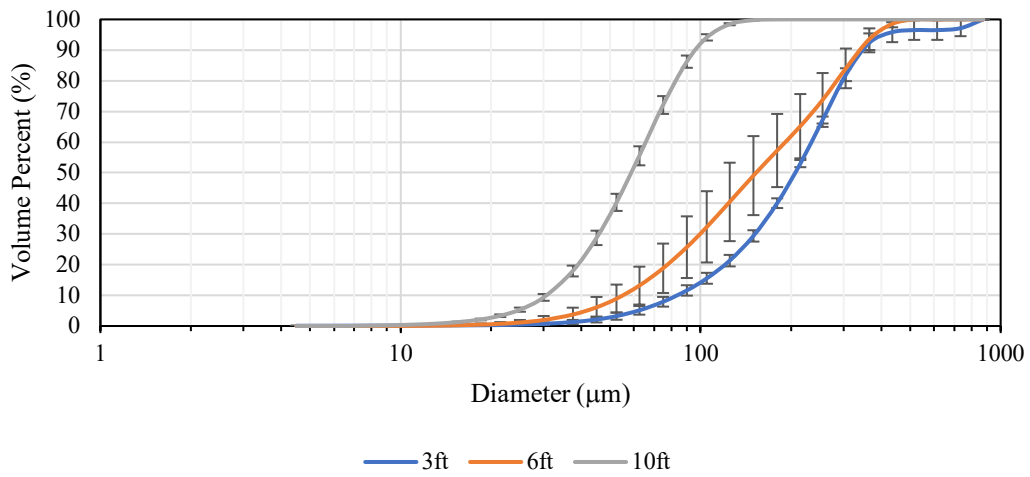
Garden sprayer Cumulative Distribution DI
