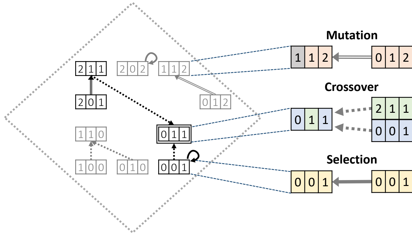
(b) Genetic Algorithm
