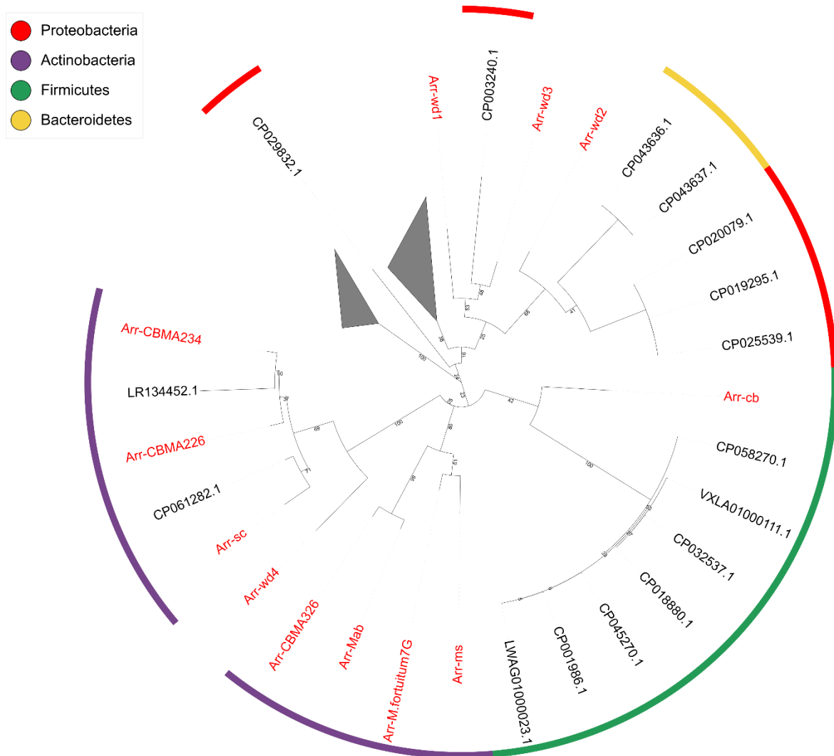
Figure S1: Plasmid Arr phylogeny generated by the maximum likelihood method. Two Proteobacteria clusters were collapsed, one with 273 sequences (including Arr-2 to Arr-8), and the other with 35 sequences. Bootstrap values above 50 are shown. The reference sequences are labelled in red and have been functionally characterized.
