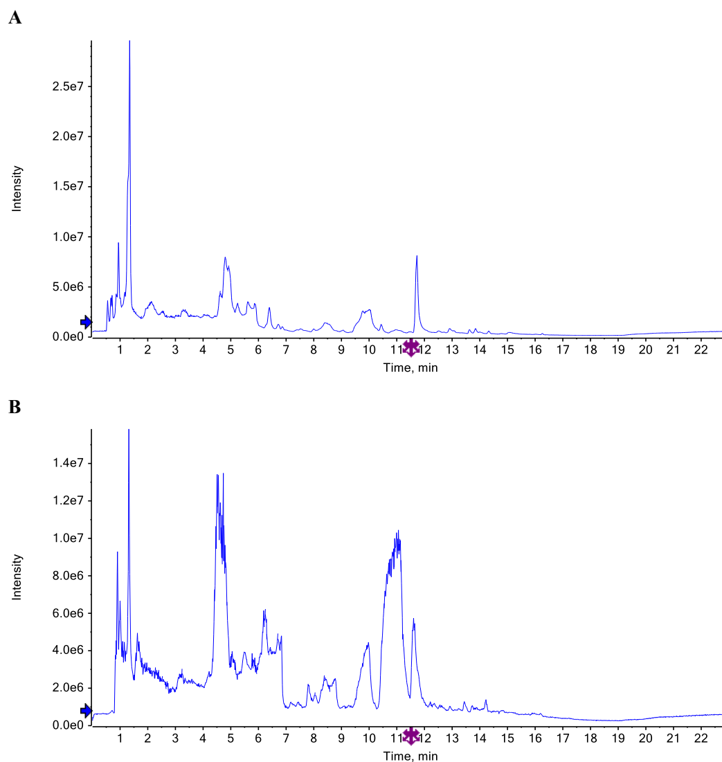
FIGURE S1 The total ion chromatogram (TIC) of metabolites determined by UHPLC-Q-TOF-MS in DN (A) and DS (B) rice. DN is rice without salt treatment, and DS is salt-tolerant rice under salt stress.
