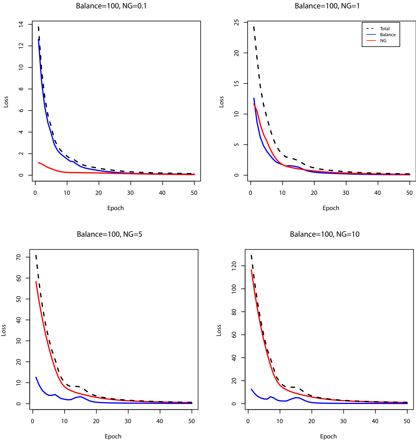
Supplementary Figure S7 Convergency of the flux balance loss and non-negative loss during the training of scFEA on the pancreatic cancer cell line data. The hyper parameters of the two loss were set differently to form four experiments. The flux balance loss, non-negative loss and total loss were blue, red and black-dash colored.
