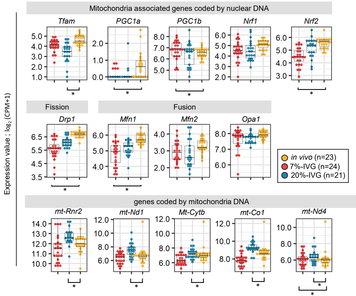
Figure S2 Expression of mitochondria-associated genes
