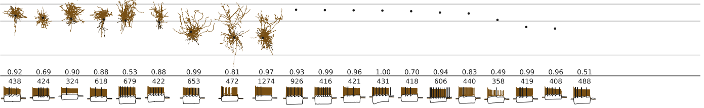
Sst C1ql3_1
