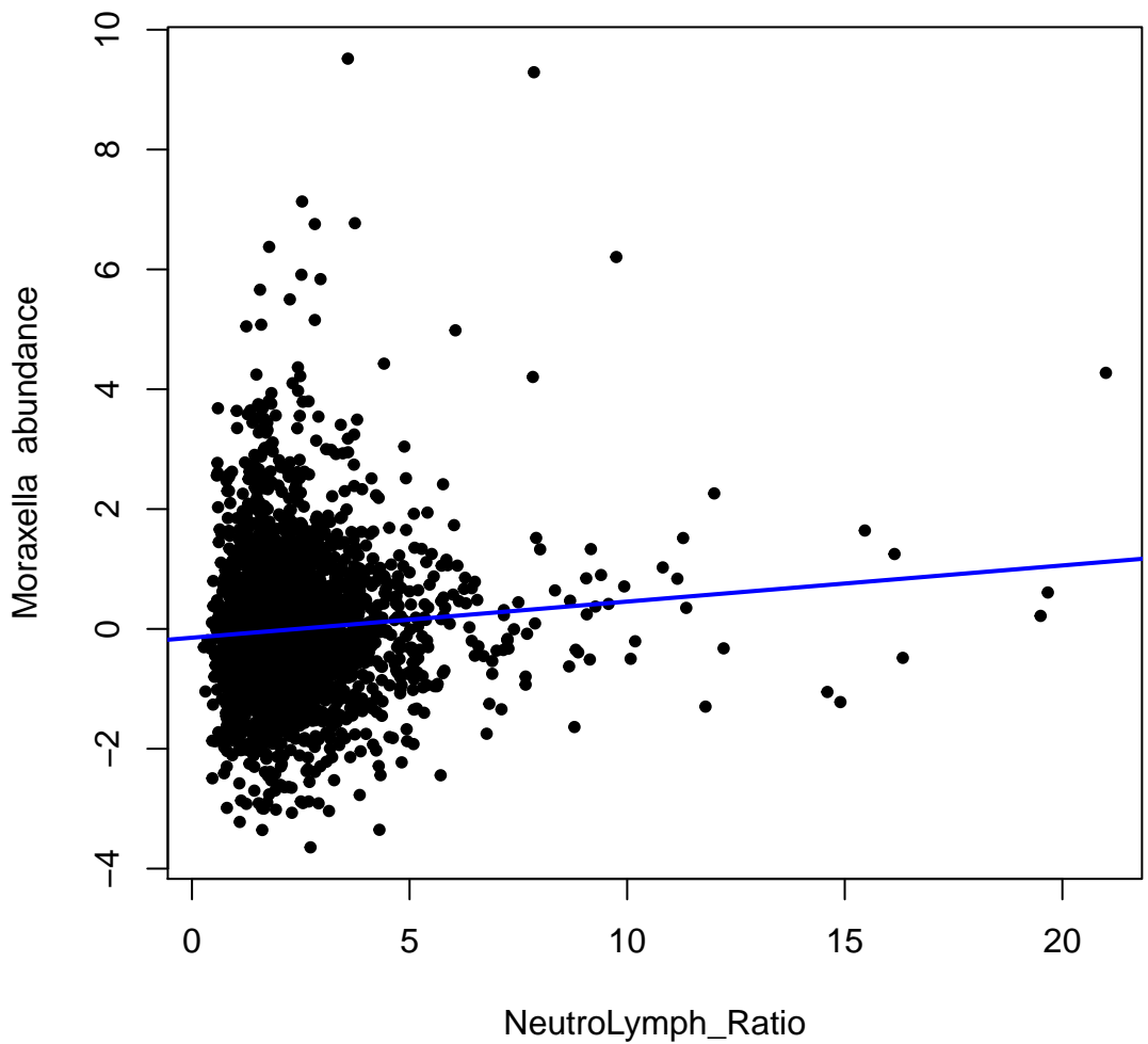
Plot of model residuals
