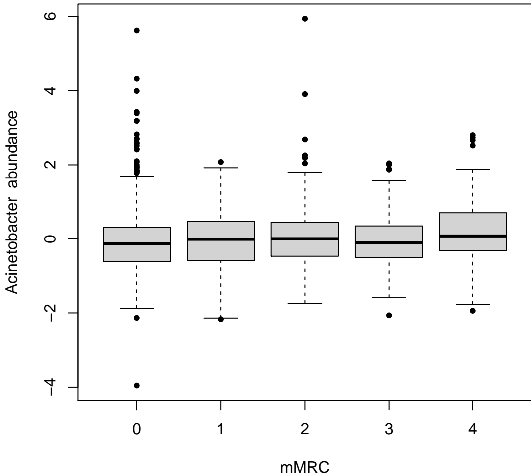
Box plot of model residuals
