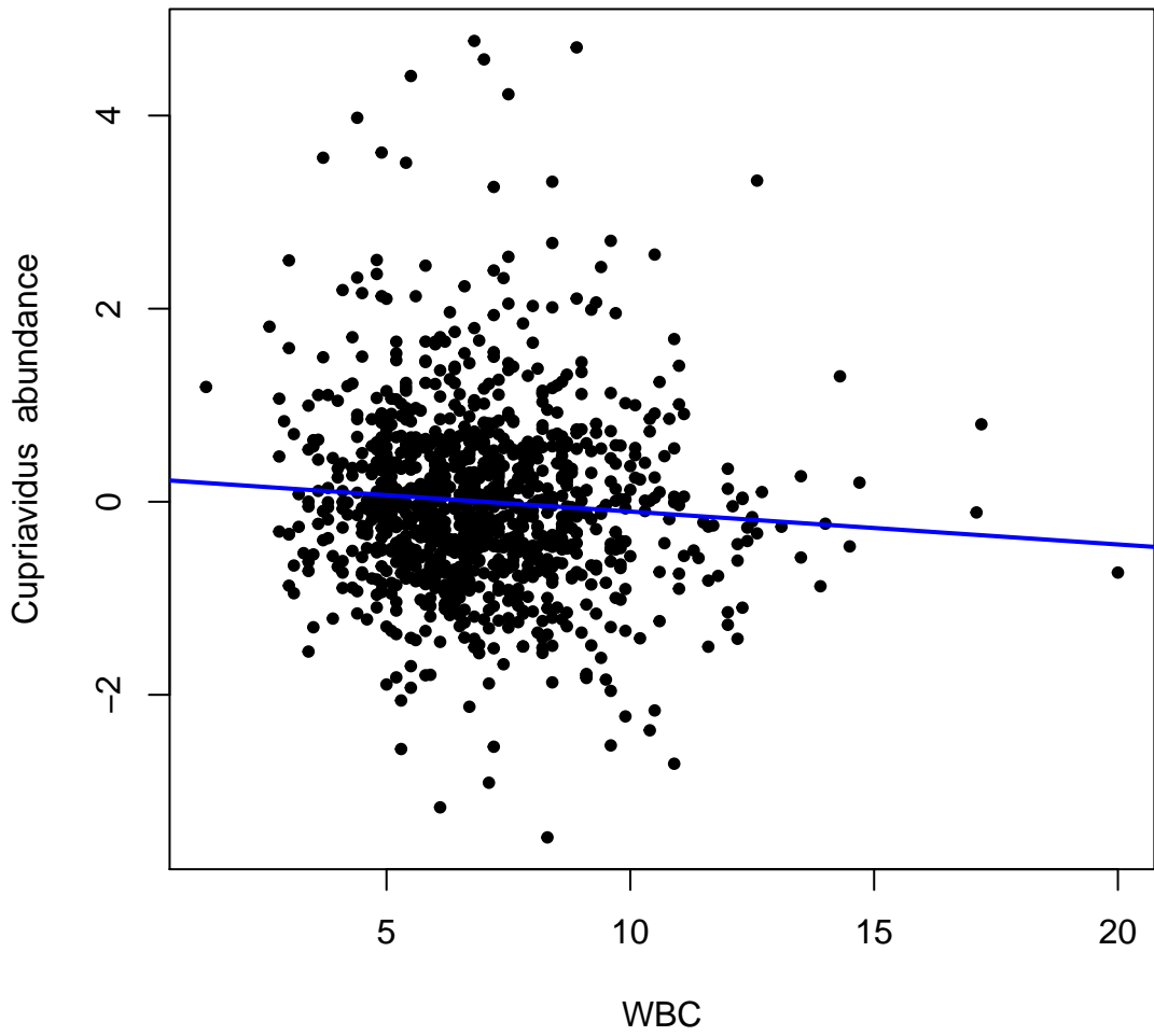
Plot of model residuals
