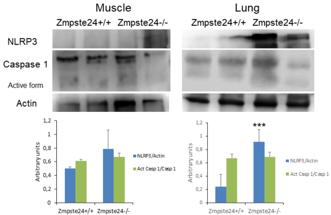
Figure EV1. NLRP3 inflammasomes expression in lung and muscle from progeroid animals.
