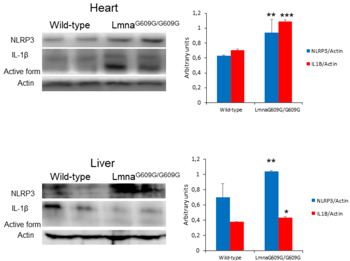
Figure EV2. NLRP3 inflammasomes expression in heart and liver from Lmna G609G/G609G mice.
