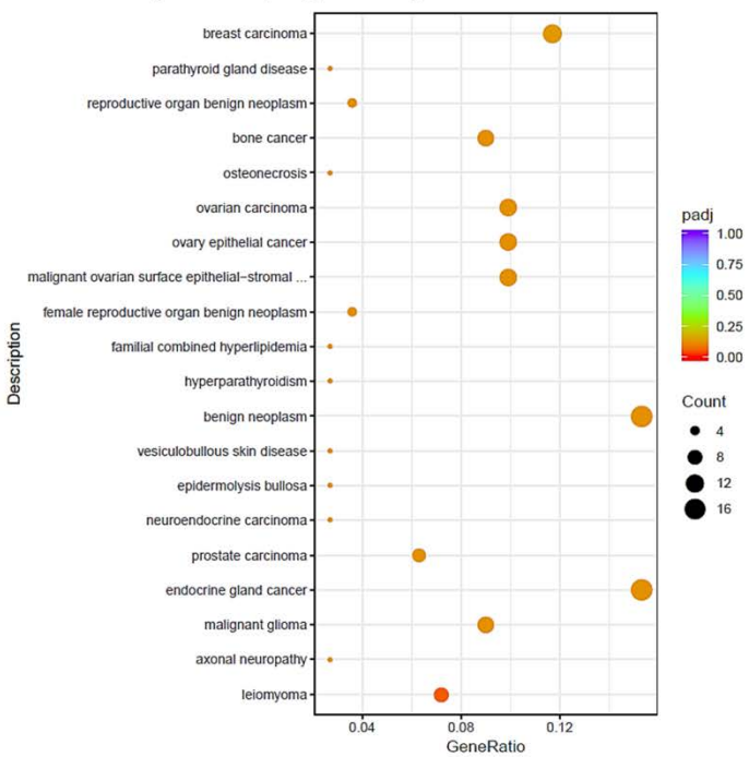
Additional file 2: Figure S1. Gene Ontology (GO) and Disease Ontology (DO) analysis of DEGs.
