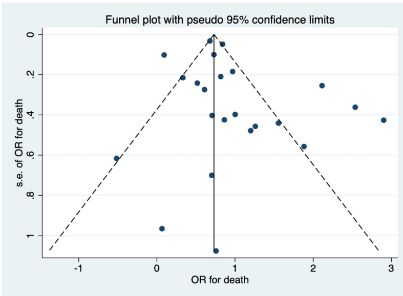
Supplementary Figure S1. Funnel plot for studies investigating the outcome of death
