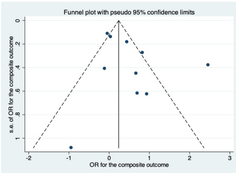
Supplementary Figure S2. Funnel plot for studies investigating composite outcomes
