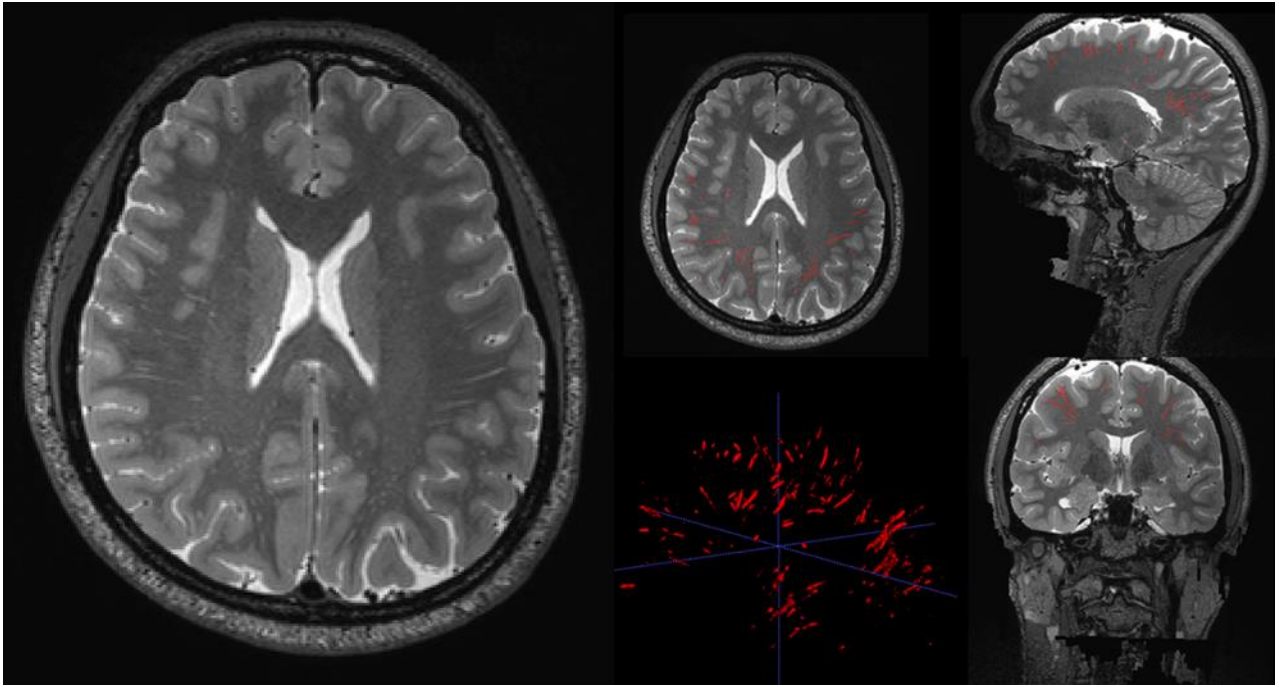
Supplementary Fig 1. Showing T2 image of a healthy adult (age 37 y-o) with extensive PVS visible. Figure on the right shows the segmented PVS mask.
