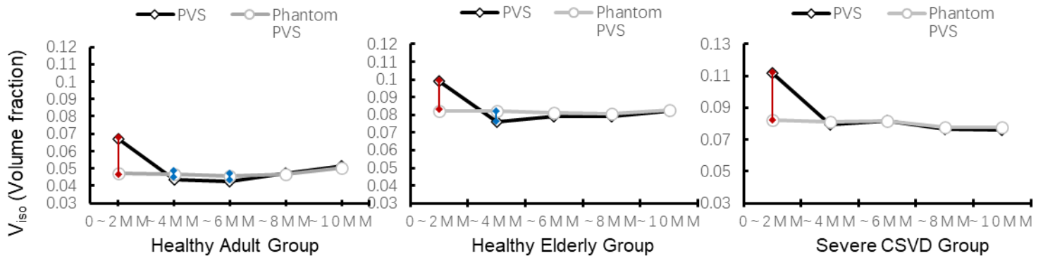
Supplementary Fig 2. Showing results for 5 layers with thickness of 2mm. For healthy elderly group, there is a significant decrease of "iso" water around 2~4mm of PVS. And in the CSVD group the decrease of "iso" water is not significant (Previously we find this decrease is significant but weaker than the other group, now it is not significant). Red lines denote Viso is significantly higher around the dPVS than around the control in that specific layer between the connected pair, and blue line vice versa.
