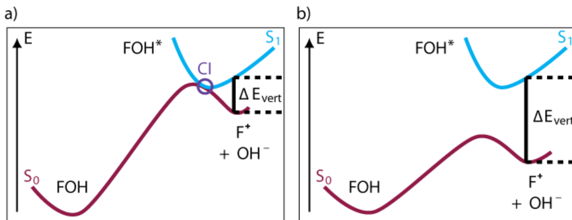
Figure S8: Illustration of computational screening procedure for fluorene-like (FOH) compounds adapted from Winter et al. [7] A productive photocage a) is photoexcited (FOH*) from the electronic ground state S 0 to the first singlet excited state S 1 and arrives in the product state (F + + OH - ) via a conical intersection (CI). This is possible due to a stabilized excited state and an energetically high lying product state. As such, the vertical absorption energy of the product, ΔE vert , is expected to be rather small. On the contrary, an unproductive photocage b) with an energetically low product does not have a CI between S 0 and S 1 and will consequently show a large ΔE vert . Thus, the smaller ΔE vert , the more likely is the existence of a productive CI channel for efficient uncaging.
