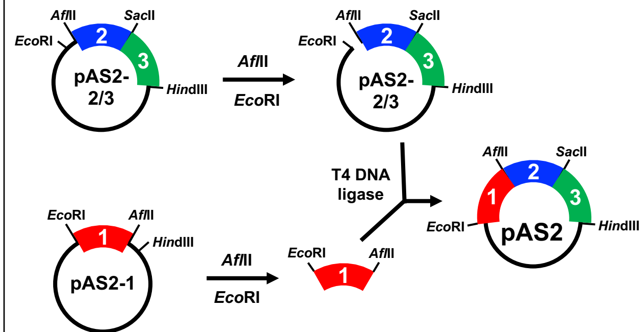
Additional File 1. Stepwise cloning scheme for ASncmtRNA-2. Colors of inserts cloned into pUC57 are the same as the corresponding RNA segments shown in Figure 1A. Only pertinent restriction sites are shown.
