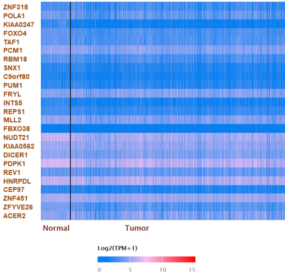
Supplementary Figure 1. Analyzed some genes positively related to ZNF304 expression in ccRCC tissues from the TCGA database.
