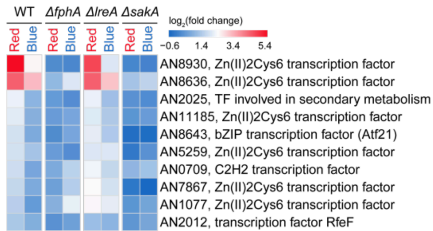
Fig. S6: Heatmap of nopA , cryA (A), top 10 light-regulated transcription factors (B) upon red and blue light in different strains. The colors of heatmap represent log 2 (fold change) of DEGs. Range of log 2 (fold change) is indicated in the color bar.
