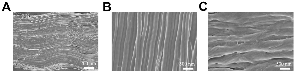
Supplementary Figure 1. The microstructures of collagen membranes. (A) The SEM images of lateral view of untreated collagen membrane. (B) The SEM images of surface view of untreated collagen membrane. (C) The SEM images of surface view of gelatin.
