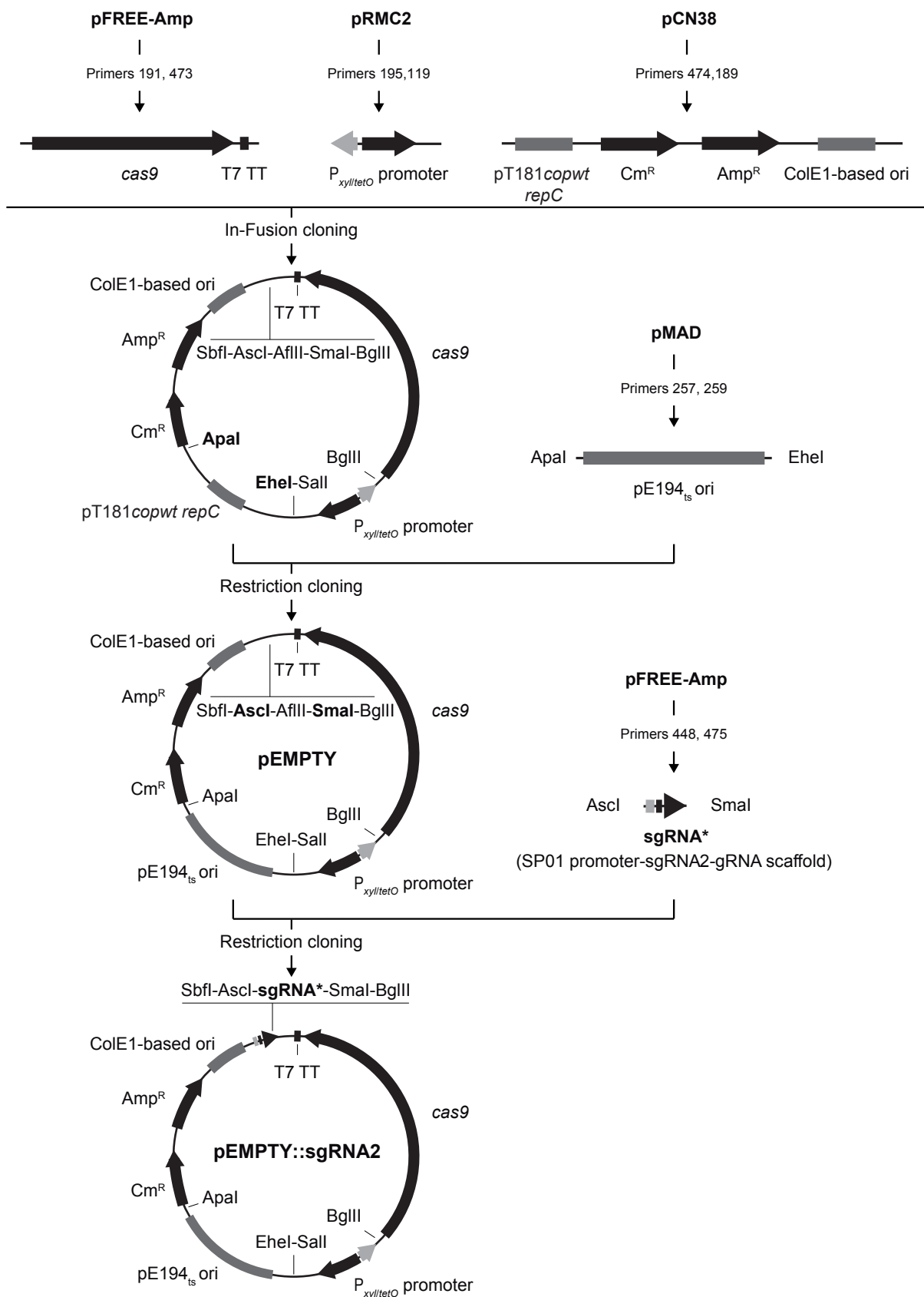
Fig. S1. Schematic representation of the construction of the pEMPTY::sgRNA2 plasmid.
