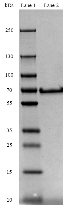
Figure S2: SDS-polyacrylamide gel showing the purification of Nd-XoxF1 from Methylacidimicrobium thermophilum AP8. Lane 1: 3 \mu L PageRuler Plus Prestained Protein Ladder protein ladder of different masses in kDa. Lane 2: 2 \mu g purified Nd-XoxF1 stained with Coomassie Brilliant Blue.
