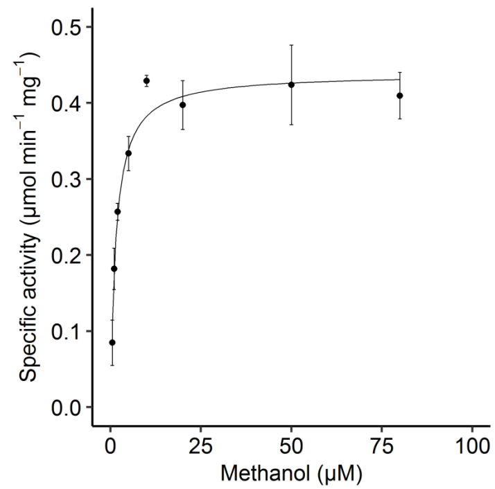
Figure S4: Specific enzyme activity of methanol oxidation by Nd-XoxF1 measured spectrophotometrically in a 4 mL cuvette.
