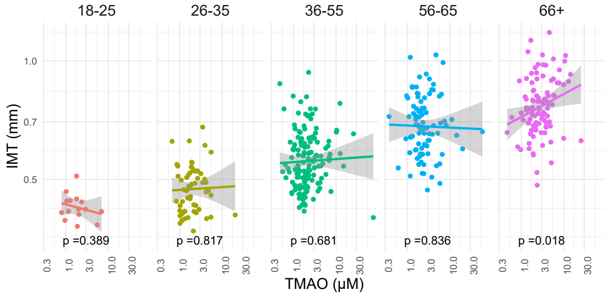
Figure S1. Associations between carotid intima–media thickness and TMAO plasma concentration by age groups.
