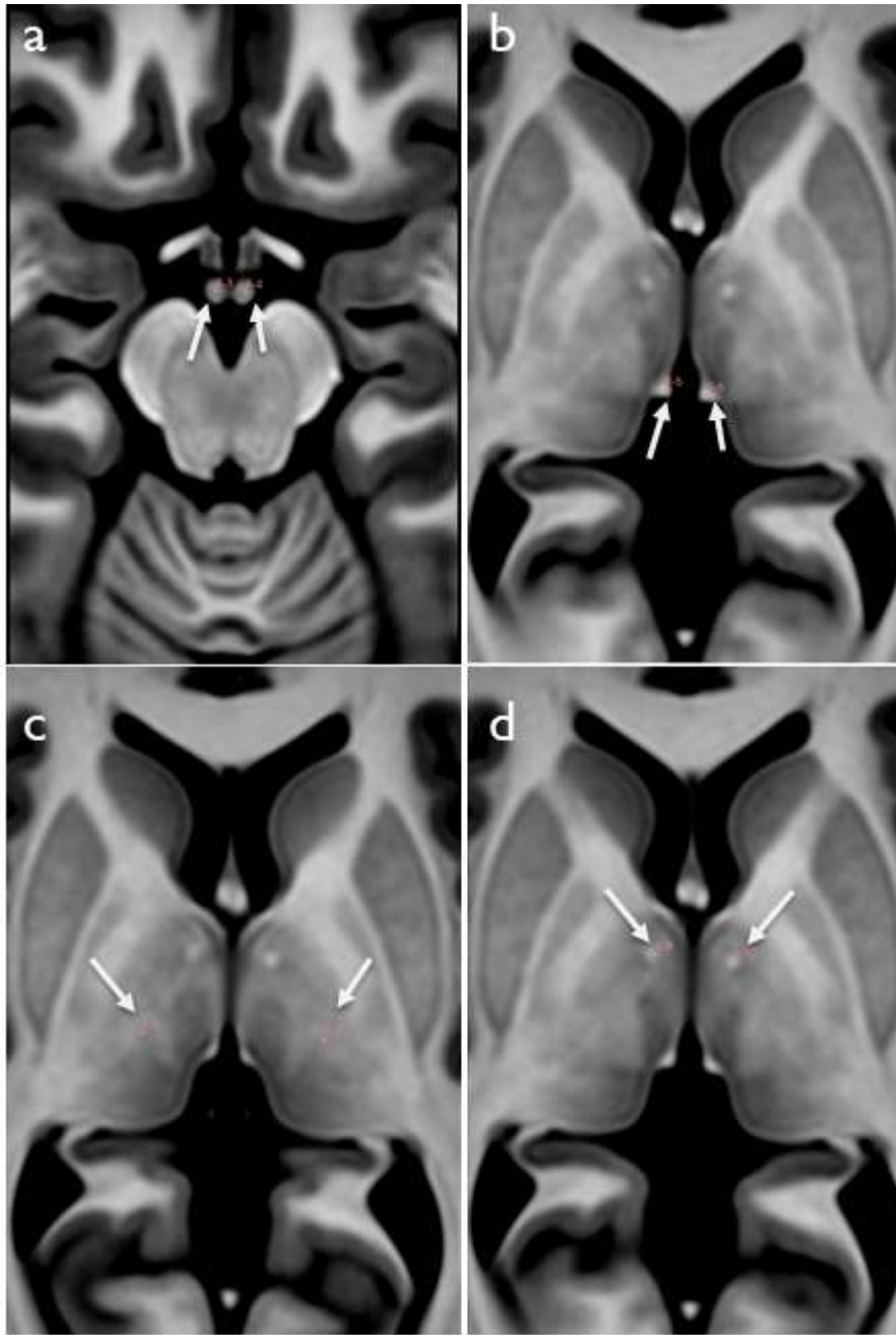
Supplementary Figure 1. Anatomical landmarks used to validate the custom template to MNI nonlinear registration- mammillary body (a), left and right habenula (b), left and right pulvinal peak (c), and left and right mammillothalamic tract (d). The anterior and posterior commissure were also used but are omitted here for brevity.
