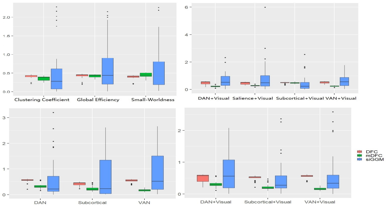
Figure 9. Prediction box plots for BDI adjusted analysis with network density = 0.15
