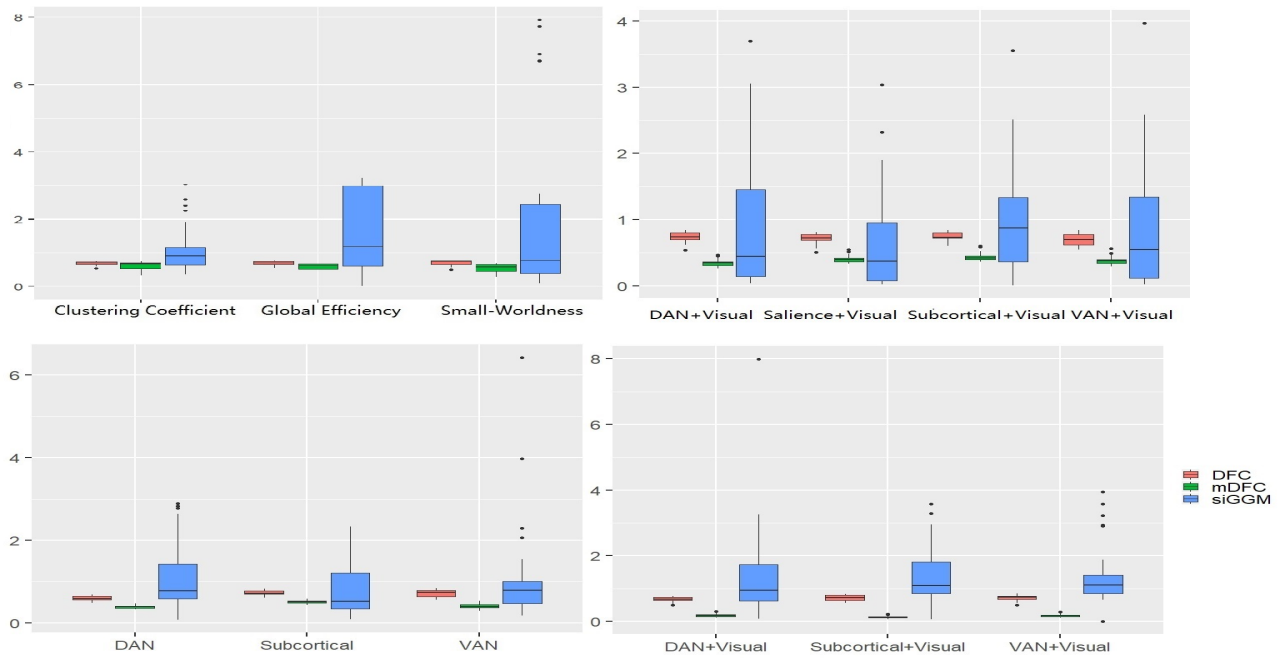
Figure 8. Prediction box plots for BDI unadjusted analysis with network density = 0.05
