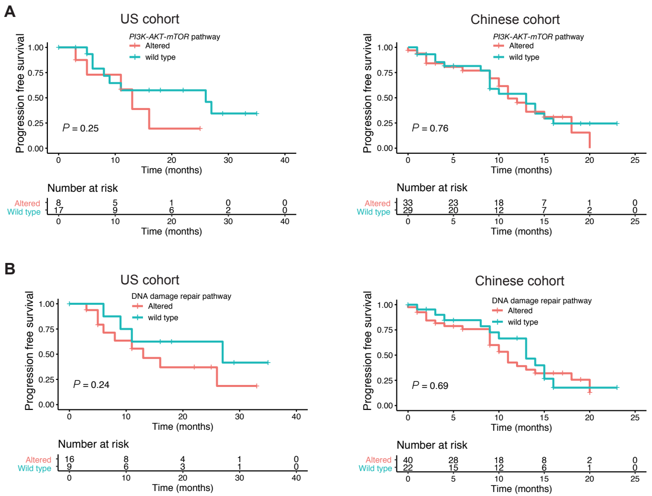
Supplementary figure 1. Survival analysis of Chinese and US patients. A , Progression free survival (PFS) of patients with or without PI3K-AKT-mTOR pathway alteration. B , PFS of patients with or without DNA damage repair pathway alteration. P value was calculated using log-rank test.
