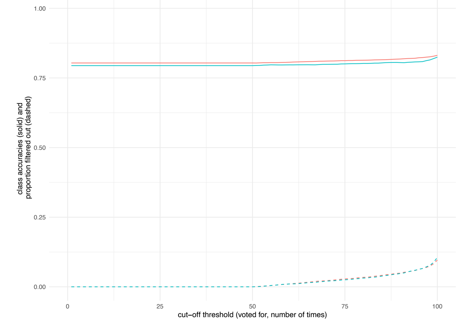
counting
