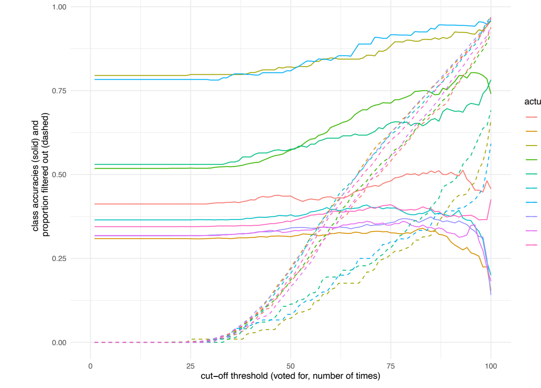
counting
