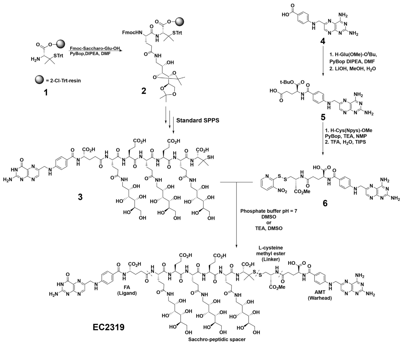
Figure 1. Chemical structures and total synthesis
