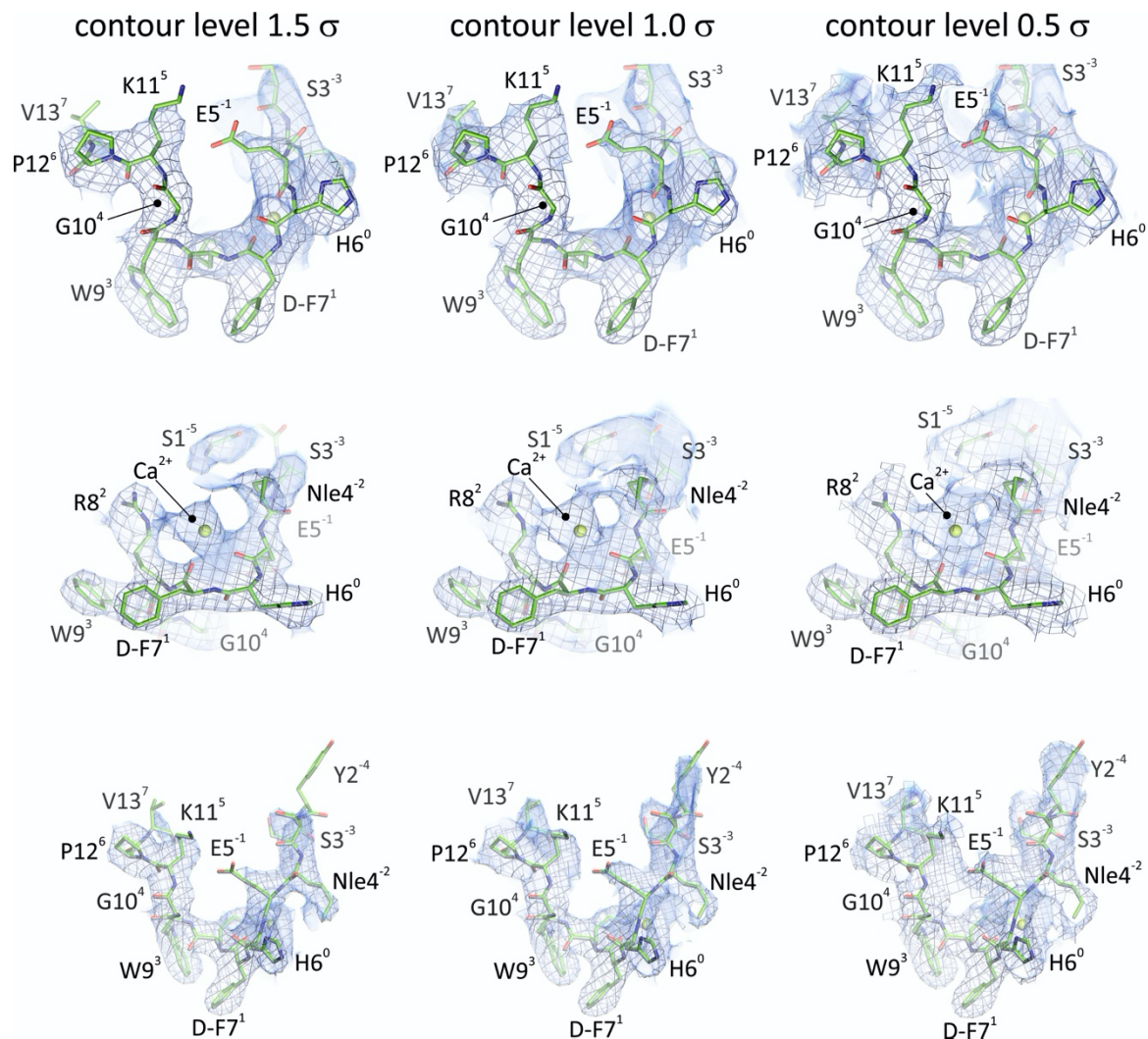
Fig. S7: Quality of the cryo-EM density map of the NDP- \alpha -MSH ligand in the NDP- \alpha -MSH-MC4R-Gs-Nb35 complex. Three different views (top to bottom) on the NDP- \alpha -MSH ligand (green color) together with the coordinating calcium ion (lemon green color). All figures show cryo-EM densities of the ligand (light blue colored mesh/volume) contoured at three different contour levels (1.5 (left), 1.0 (middle) and 0.5 \sigma (right)). NDP- \alpha -MSH is depicted as sticks and the calcium ion as sphere representation.
