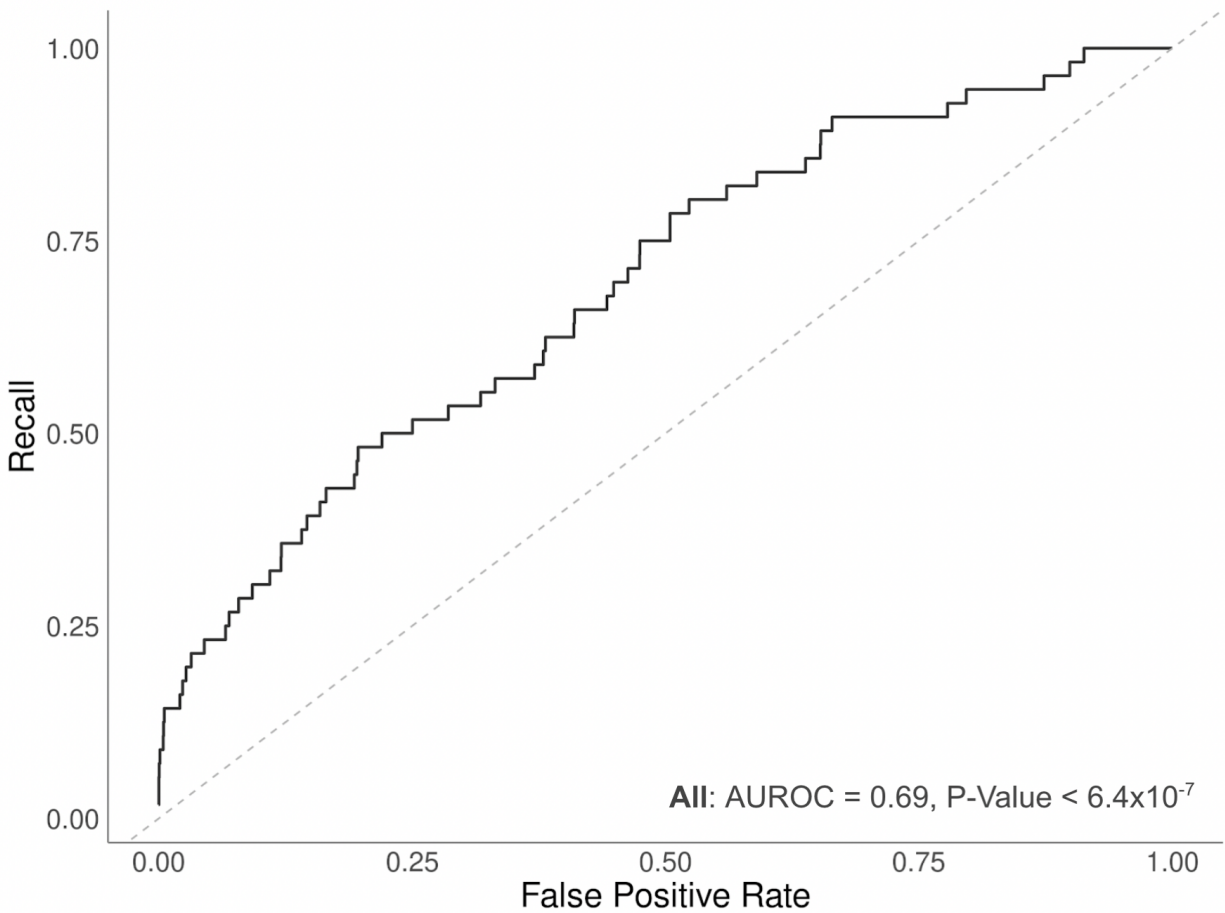
S15 Fig. Enrichment of all curated PAX6/Pax6 targets among differentially expressed genes in Walcher et al., 2013 [1]. AUROC and the corresponding p-value (Mann-Whitney U Test) are displayed in the panel.
