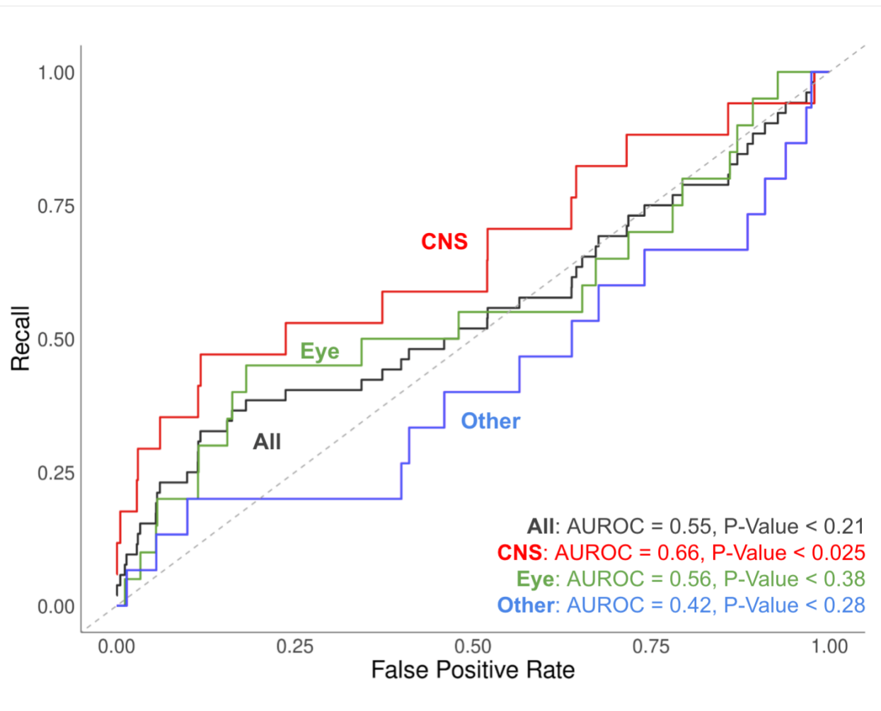
S20 Fig. Enrichment of curated PAX6/Pax6 targets among differentially expressed genes in Narayanan et al., 2018 [1] by tissue types. AUROCs and the corresponding p-values (Mann-Whitney U Test) are displayed in the panel. Color coding corresponds to categories of targets. Only the targets experimentally verified in the CNS show statistically significant enrichment.
