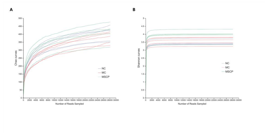
Supplementary Figure 1. Alpha diversity indexes of microbiota in different groups. (A) Chao diversity index. (B) Shannon diversity index.
