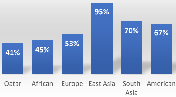
rs6629110 - ACE2
