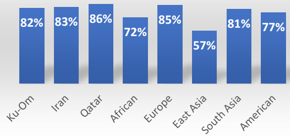
rs42398-C-T ERAP1
