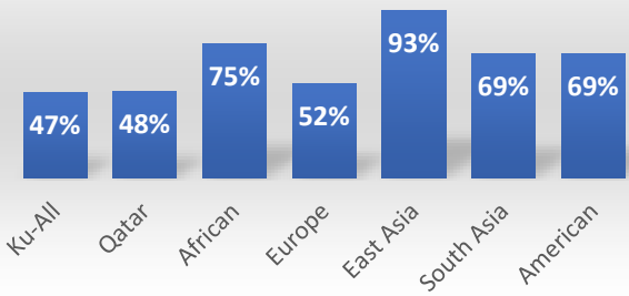
rs4060 - ACE2
