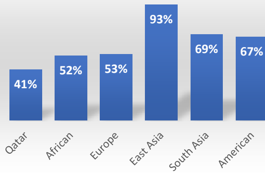
rs6632704 - ACE2
