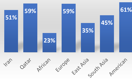
rs27039-G-A ERAP1
