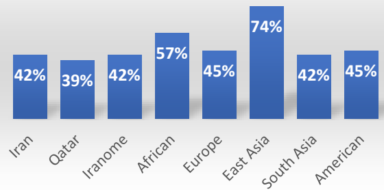
rs1996225 - ACE2
