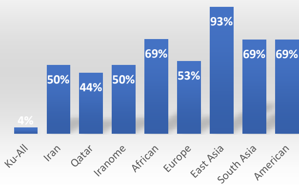
rs4060 - ACE2
