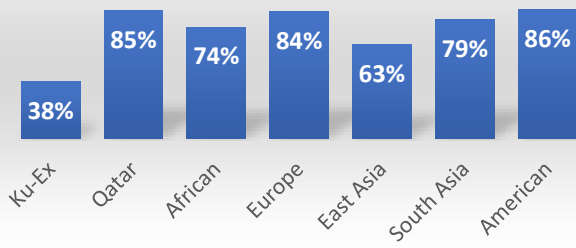
rs27433-T-G ERAP1
