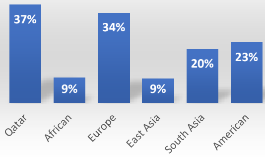
rs7356594-G-T ERAP1
