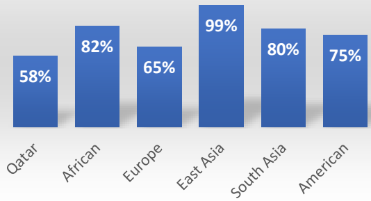
rs6632704 - ACE2
