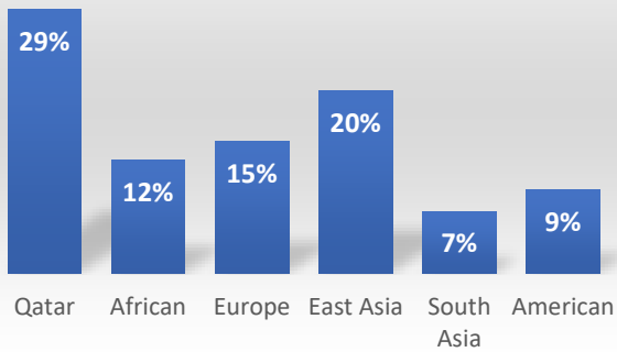
rs3095257-G-T HLA-B
