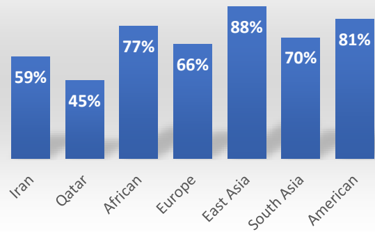
rs2523663-G-T HLA-B
