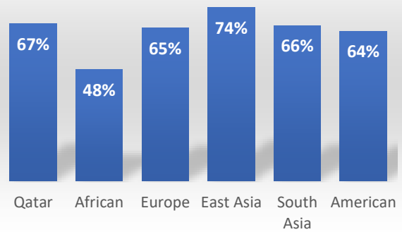
rs27039-G-A ERAP1
