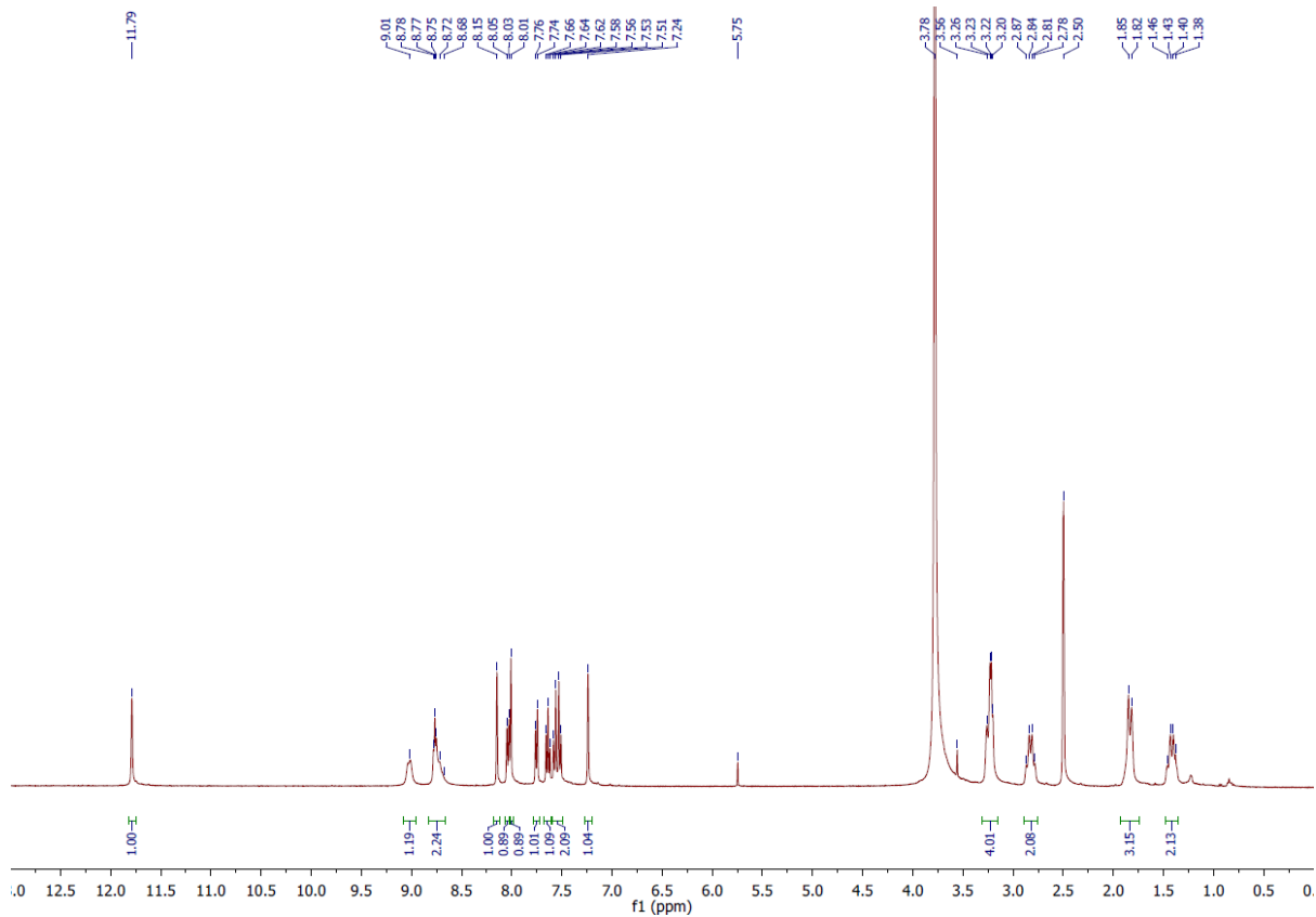
46. 5-(3-Cyanophenyl)-N-(piperidin-4-ylmethyl)-1H-indole-2-carboxamide Hydrochloride (46).
