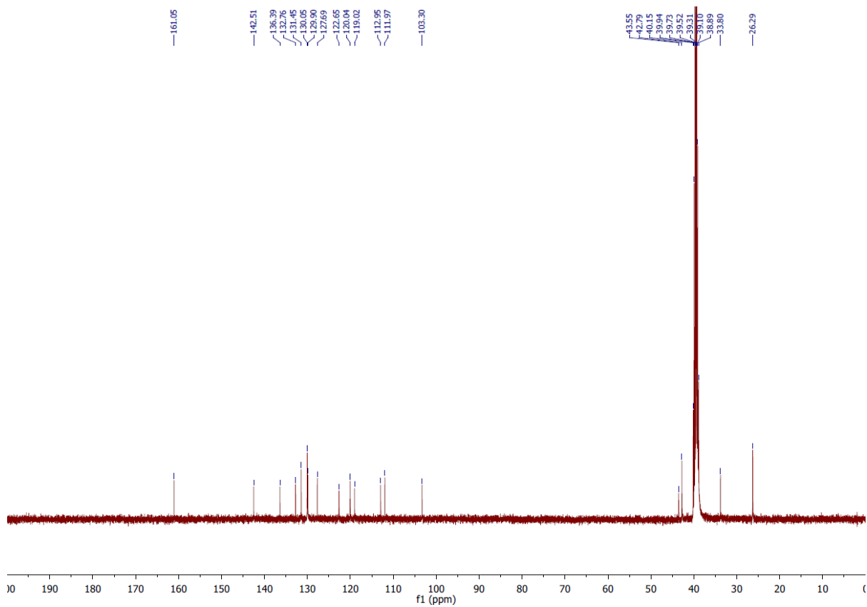
47. N-(Piperidin-4-ylmethyl)-1H-indole-2-carboxamide Hydrochloride (47).
