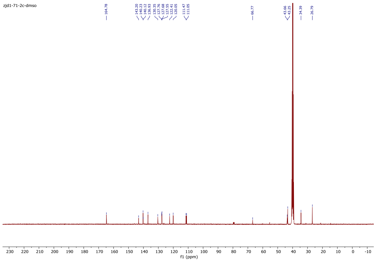
29. N-(Piperidin-4-ylmethyl)-6-(pyridin-4-yl)-1H-indole-3-carboxamide Hydrochloride (29).
