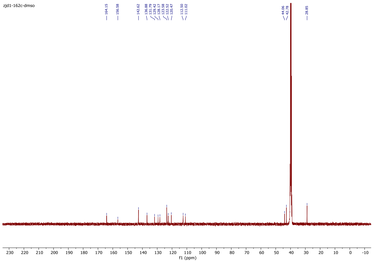
28 . N-(Piperidin-4-ylmethyl)-6-(pyridin-3-yl)-1H-indole-3-carboxamide Hydrochloride (28).
