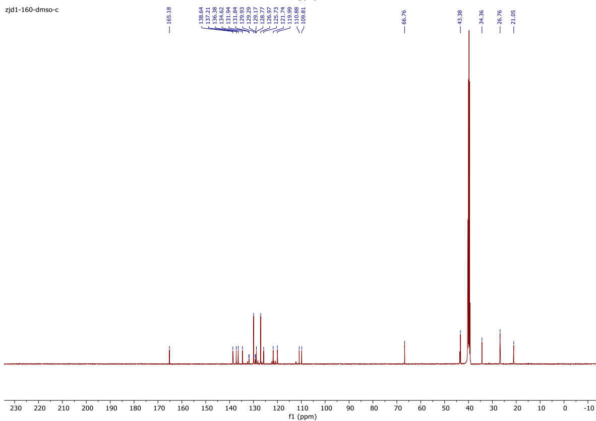
23. 6-(4-(Aminomethyl)phenyl)-N-(piperidin-4-ylmethyl)-1H-indole-3-carboxamide Hydrochloride ( 23 ).
