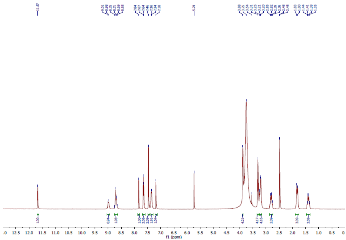
42. 5-(4-Morpholinophenyl)-N-(piperidin-4-ylmethyl)-1H-indole-2-carboxamide Hydrochloride ( 42 ).
