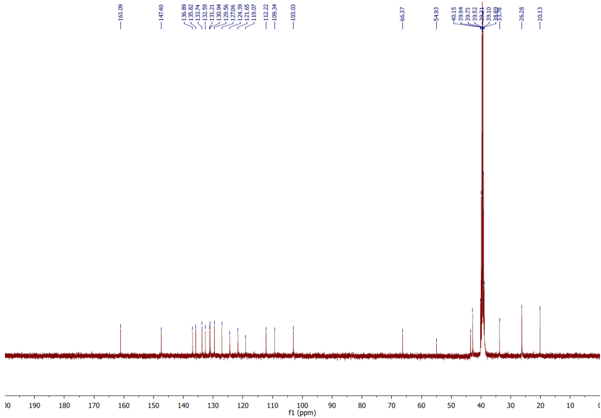
46. 5-(3-Cyanophenyl)-N-(piperidin-4-ylmethyl)-1H-indole-2-carboxamide Hydrochloride (46).
