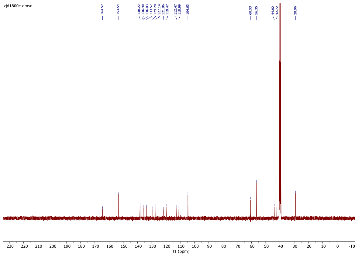
16. 5-(4-Fluorophenyl)-N-(piperidin-4-ylmethyl)-1H-indole-3-carboxamide Hydrochloride ( 16 ).
