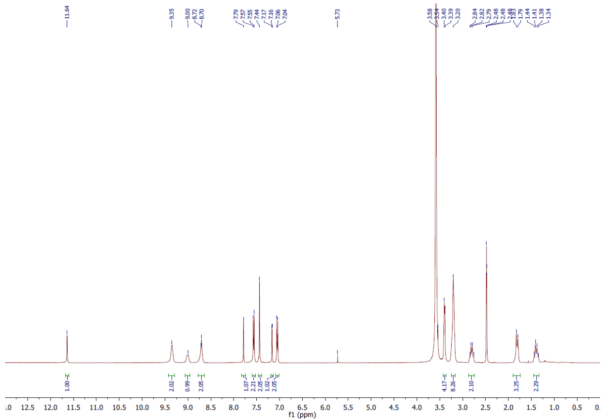
43. 5-(4-(Piperazin-1-yl)phenyl)-N-(piperidin-4-ylmethyl)-1H-indole-2-carboxamide Hydrochloride ( 43 ).
