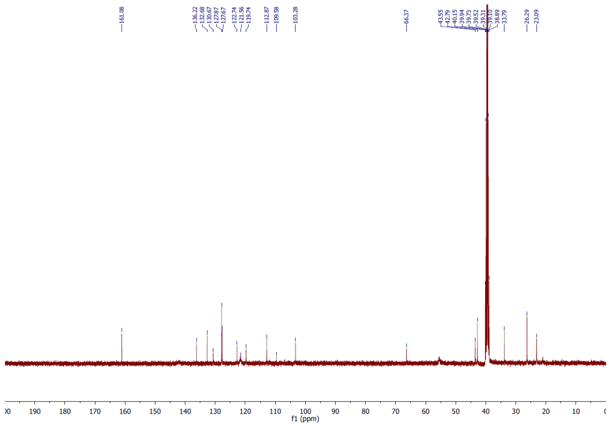
41. N-(Piperidin-4-ylmethyl)-5-(4-(pyrrolidin-1-yl)phenyl)-1H-indole-2-carboxamide Hydrochloride ( 41 ).
