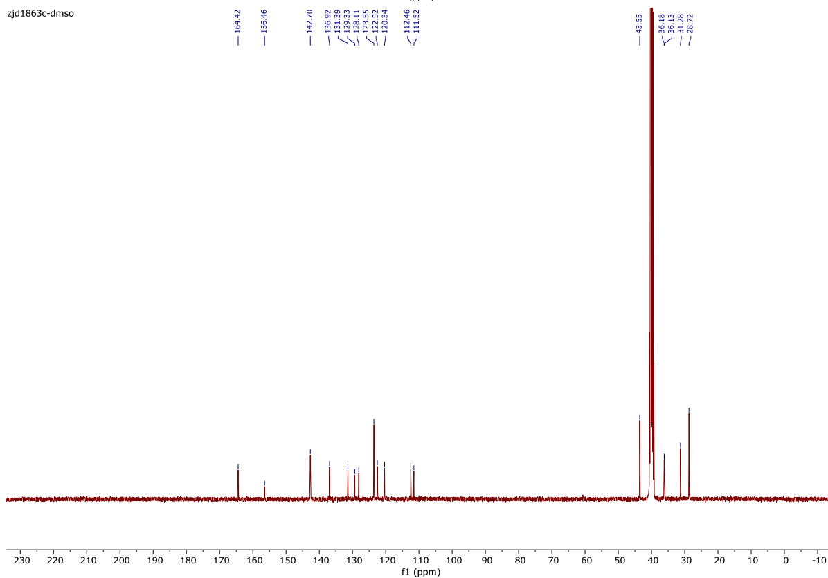
32. N-(Piperidin-4-ylmethyl)-6-(1H-pyrazol-3-yl)-1H-indole-3-carboxamide Hydrochloride (32).
