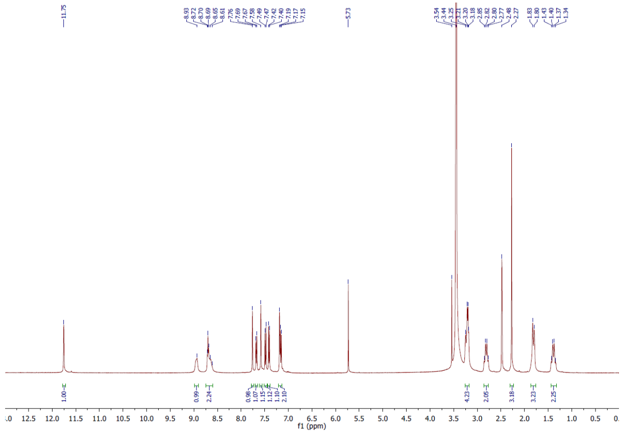
45. 5-(4-Cyano-2-methylphenyl)-N-(piperidin-4-ylmethyl)-1H-indole-2-carboxamide Hydrochloride ( 45 ).
