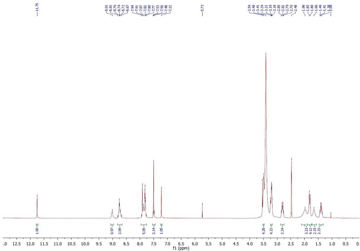
40. 5-(4-(Piperidin-1-yl)phenyl)-N-(piperidin-4-ylmethyl)-1H-indole-2-carboxamide Hydrochloride ( 40 ).
