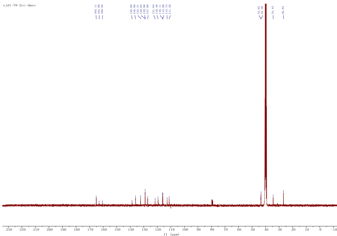
17. 5-(2,4-Difluorophenyl)-N-(piperidin-4-ylmethyl)-1H-indole-3-carboxamide Hydrochloride (17).
