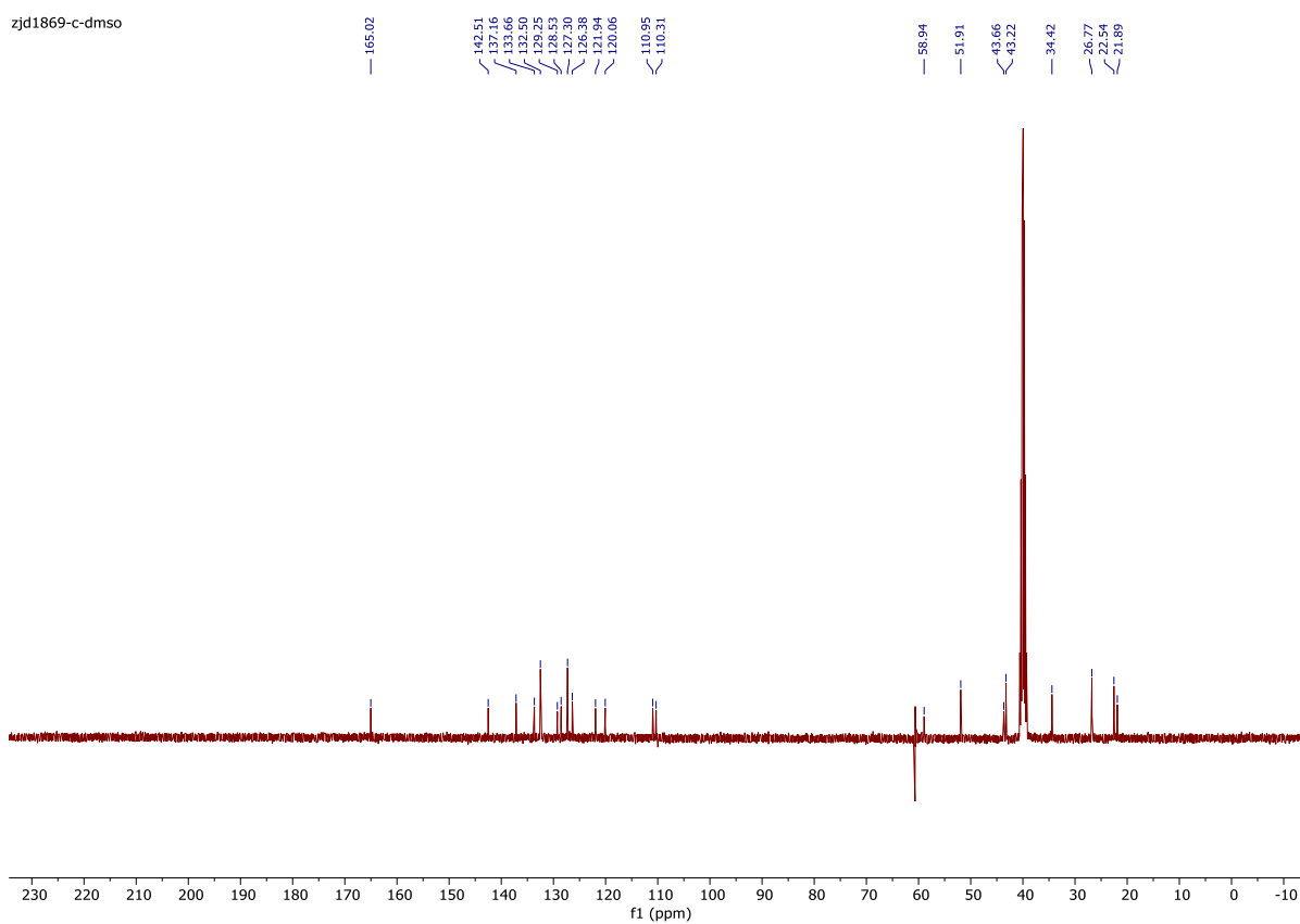
27. 6-(6-Chloropyridin-3-yl)-N-(piperidin-4-ylmethyl)-1H-indole-3-carboxamide Hydrochloride (27).
