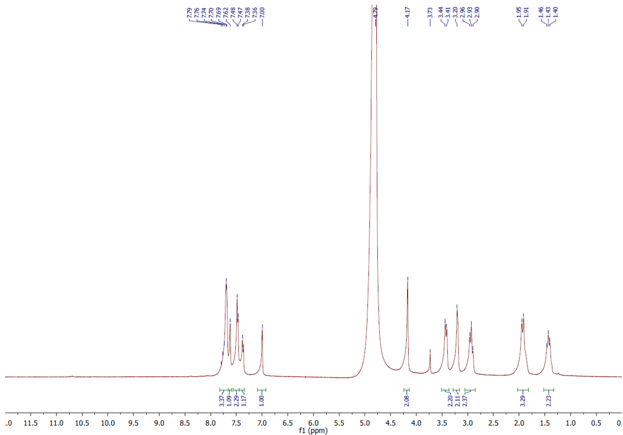
52. 6-(4-(Aminomethyl)phenyl)-N-(piperidin-4-ylmethyl)-1H-indole-2-carboxamide Hydrochloride ( 52 ).
