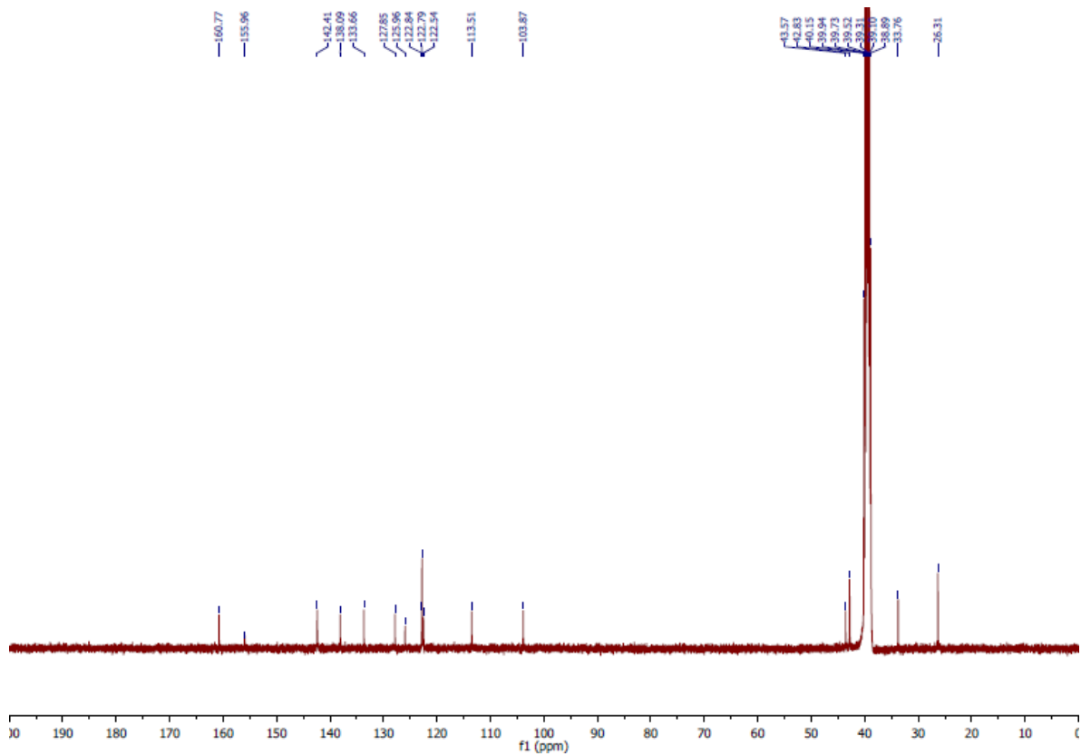
35. N-(Piperidin-4-ylmethyl)-5-(1H-pyrazol-4-yl)-1H-indole-2-carboxamide Hydrochloride
