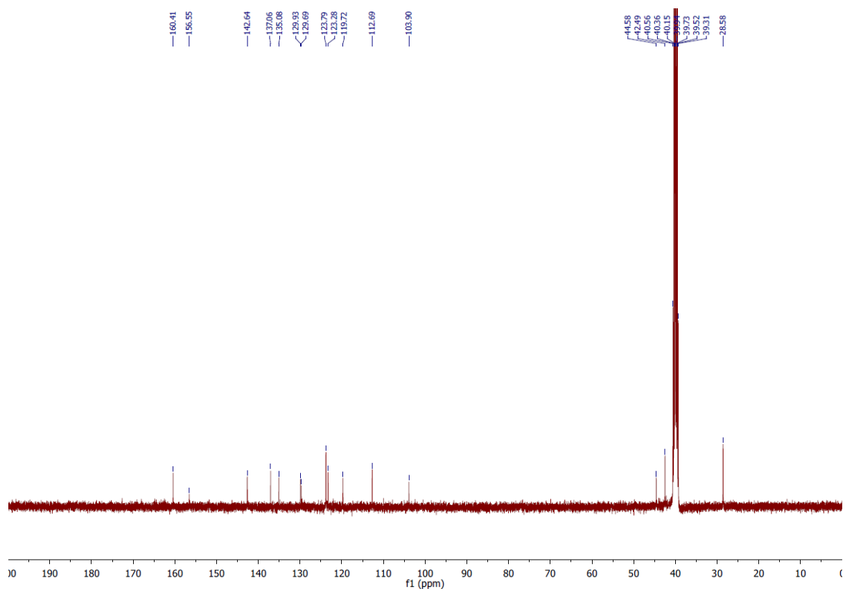
60. N-(Piperidin-4-ylmethyl)-6-(pyridin-4-yl)-1H-indole-2-carboxamide Hydrochloride ( 60 ).
