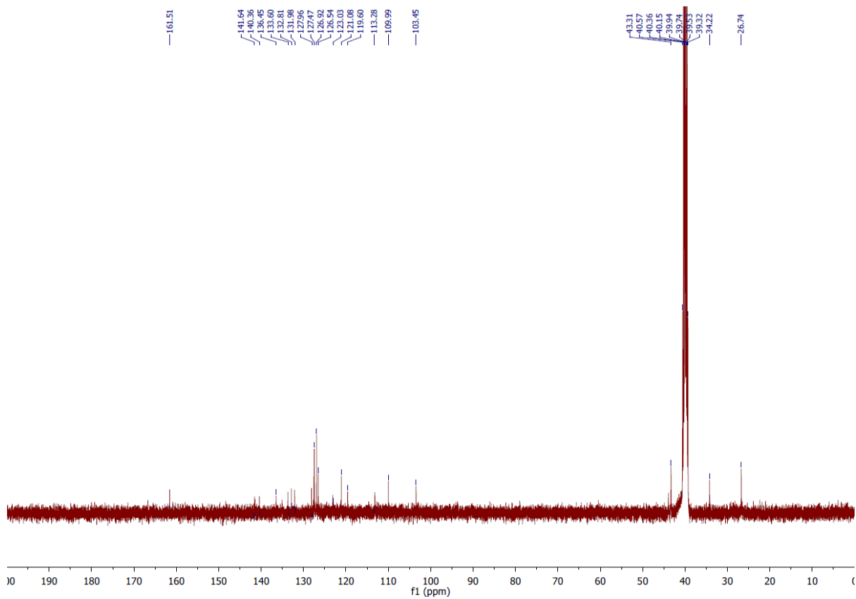
39. 5-(4-(Piperidin-1-ylmethyl)phenyl)-N-(piperidin-4-ylmethyl)-1H-indole-2-carboxamide Hydrochloride ( 39 ).
