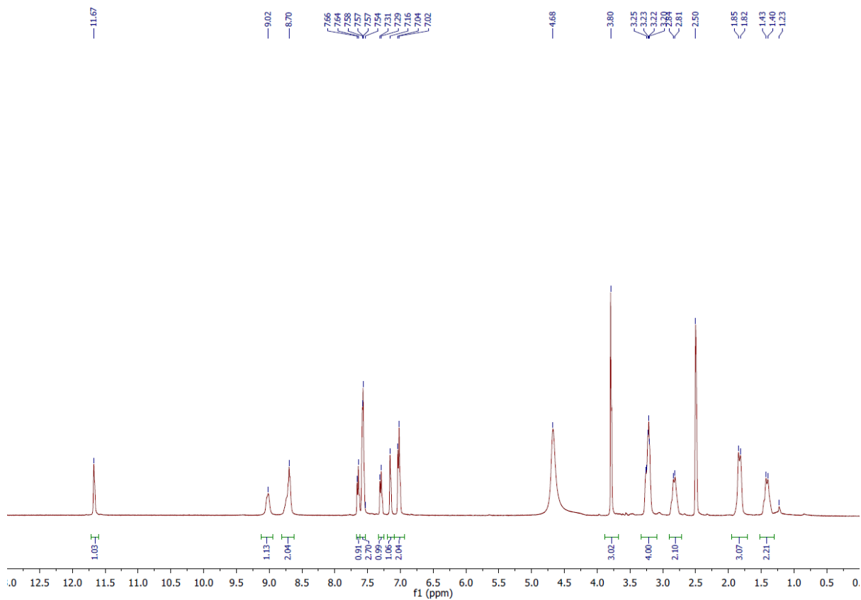
50. 6-(4-Methoxyphenyl)-N-(piperidin-4-ylmethyl)-1H-indole-2-carboxamide Hydrochloride (50).
