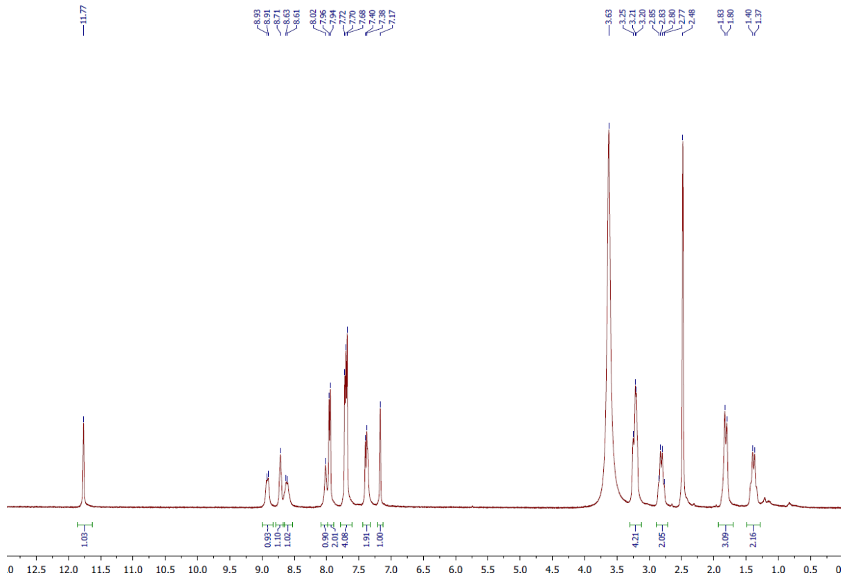
53. 6-(4-Carbamoylphenyl)-N-(piperidin-4-ylmethyl)-1H-indole-2-carboxamide Hydrochloride ( 53 ).
