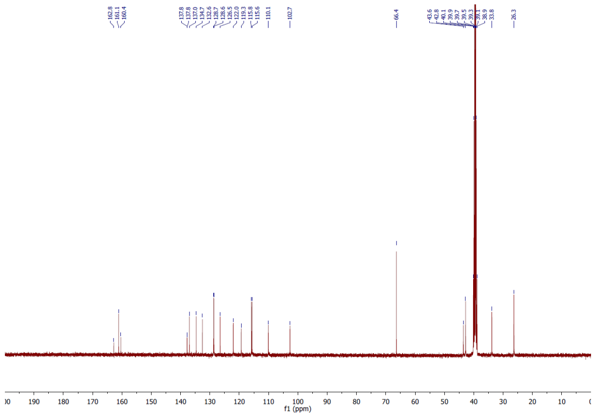
50. 6-(4-Methoxyphenyl)-N-(piperidin-4-ylmethyl)-1H-indole-2-carboxamide Hydrochloride (50).
