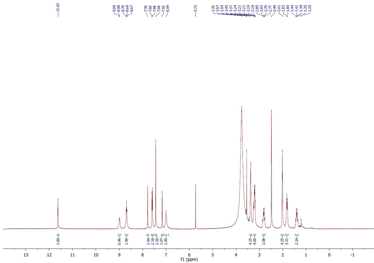
41. N-(Piperidin-4-ylmethyl)-5-(4-(pyrrolidin-1-yl)phenyl)-1H-indole-2-carboxamide Hydrochloride ( 41 ).
