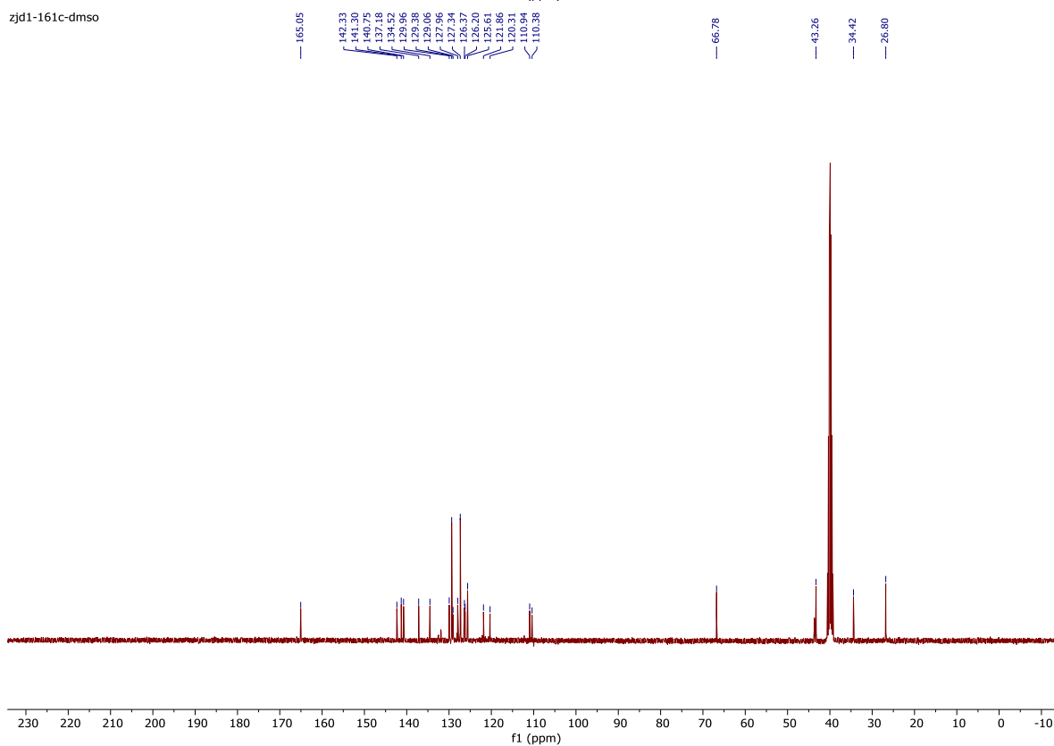
26. 6-(4-(Piperidin-1-ylmethyl)phenyl)-N-(piperidin-4-ylmethyl)-1H-indole-3-carboxamide Hydrochloride ( 26 ).
