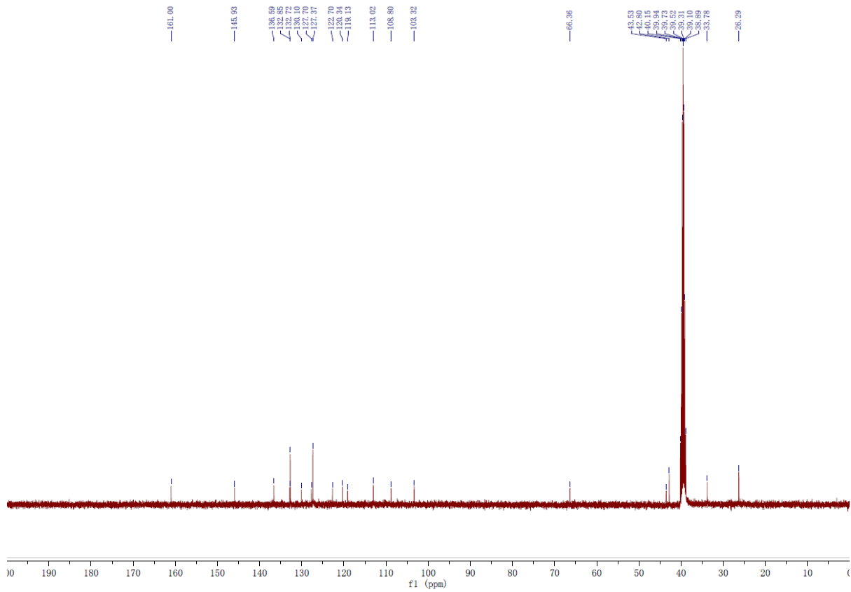
45. 5-(4-Cyano-2-methylphenyl)-N-(piperidin-4-ylmethyl)-1H-indole-2-carboxamide Hydrochloride ( 45 ).
