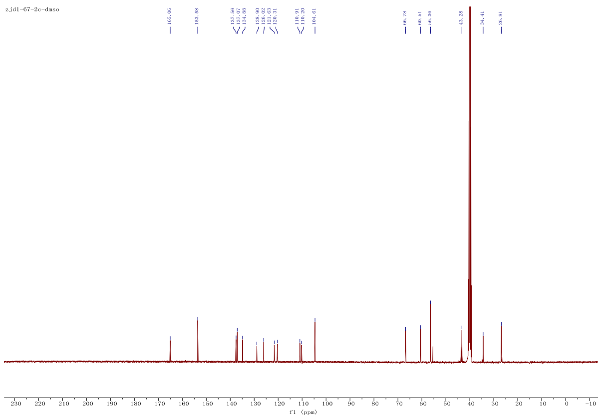
20. 6-(4-Fluorophenyl)-N-(piperidin-4-ylmethyl)-1H-indole-3-carboxamide Hydrochloride (20).
