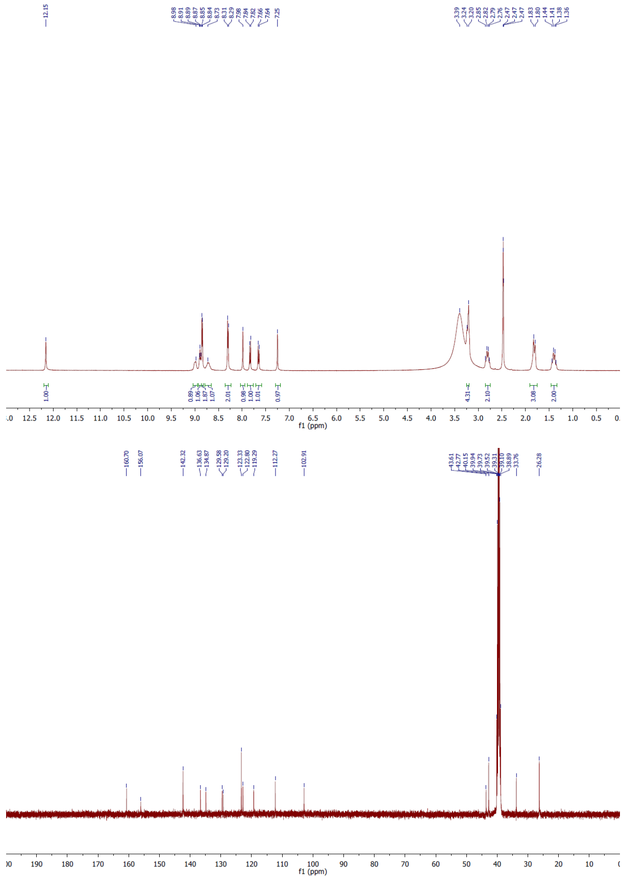
61. N-(Piperidin-4-ylmethyl)-6-(pyridin-3-yl)-1H-indole-2-carboxamide Hydrochloride ( 61 ).
