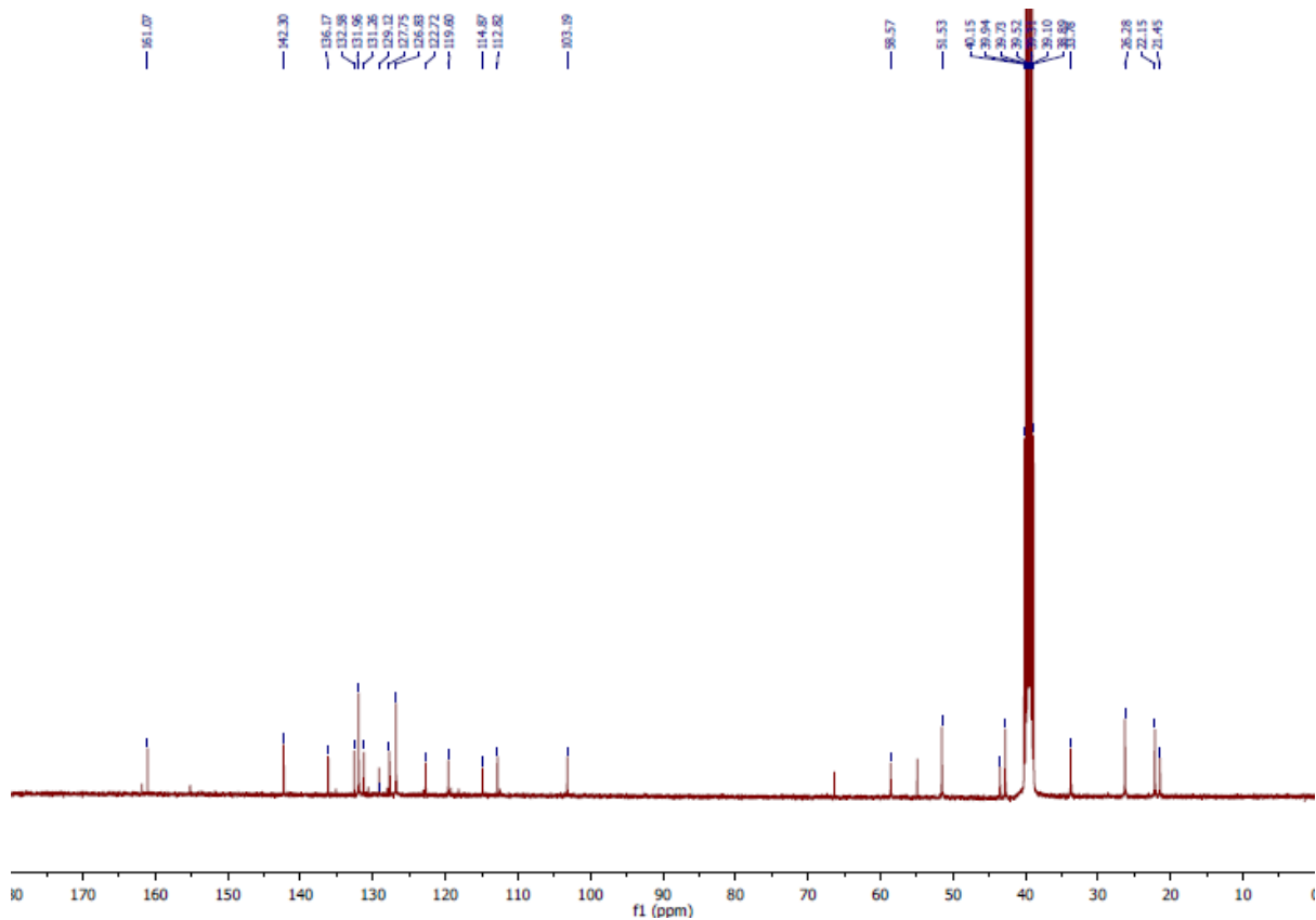
40. 5-(4-(Piperidin-1-yl)phenyl)-N-(piperidin-4-ylmethyl)-1H-indole-2-carboxamide Hydrochloride ( 40 ).
