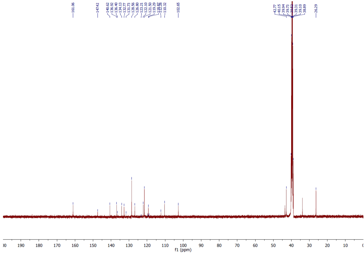
52. 6-(4-(Aminomethyl)phenyl)-N-(piperidin-4-ylmethyl)-1H-indole-2-carboxamide Hydrochloride ( 52 ).
