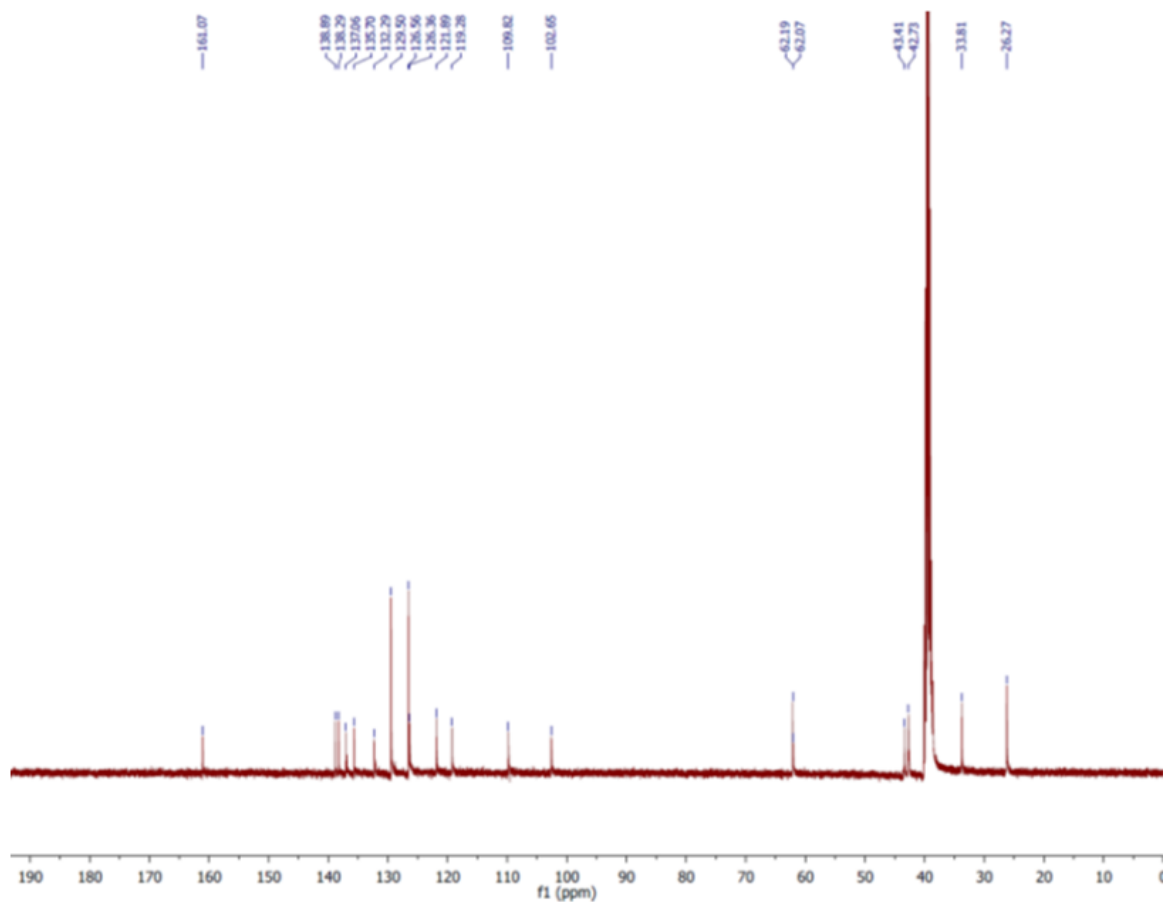
56. 6-(4-Phenoxyphenyl)-N-(piperidin-4-ylmethyl)-1H-indole-2-carboxamide Hydrochloride ( 56 ).
