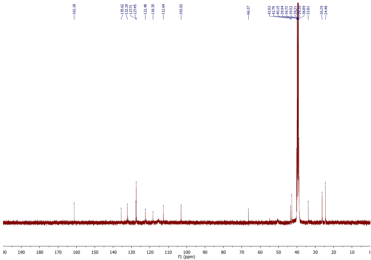
42. 5-(4-Morpholinophenyl)-N-(piperidin-4-ylmethyl)-1H-indole-2-carboxamide Hydrochloride ( 42 ).
