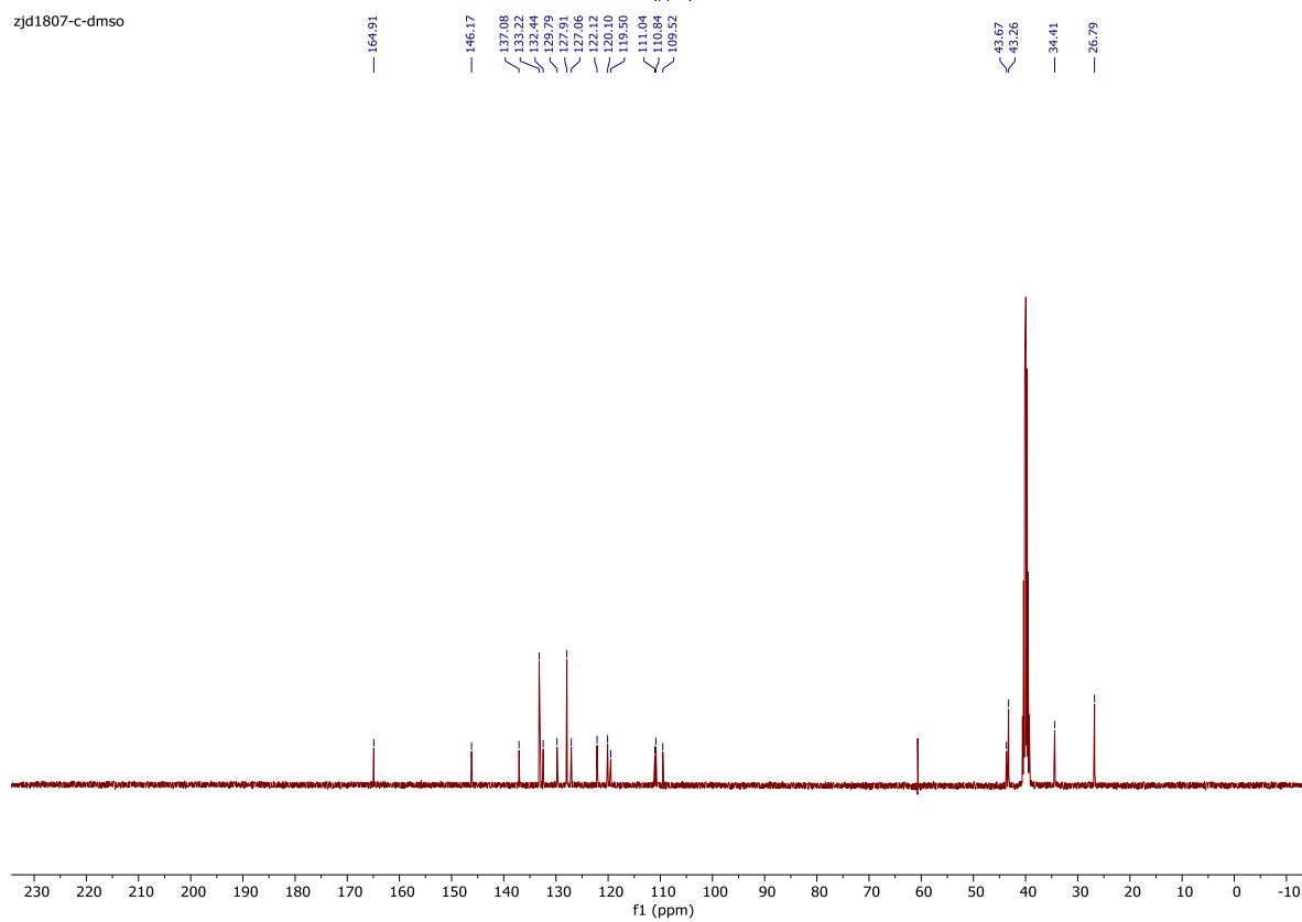
25. 6-([1,1'-Biphenyl]-4-yl)-N-(piperidin-4-ylmethyl)-1H-indole-3-carboxamide Hydrochloride (25).
