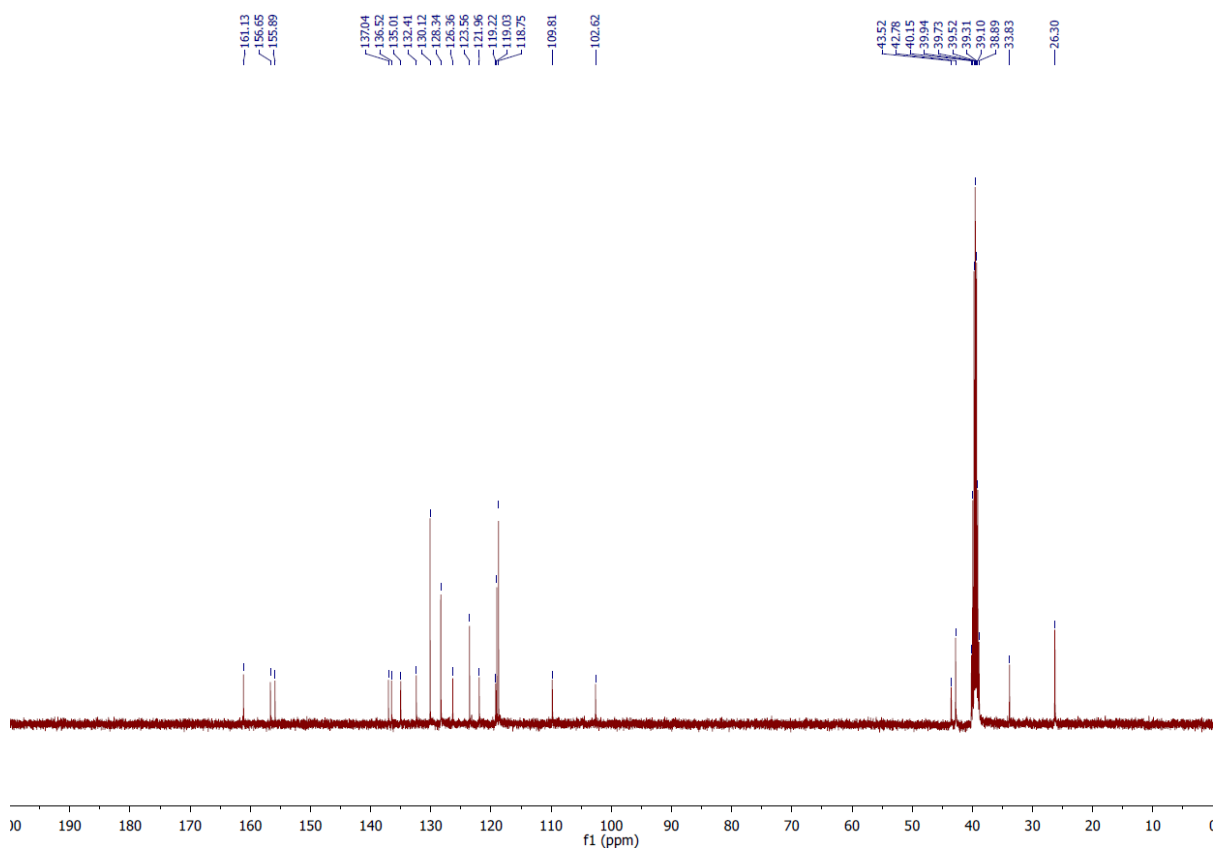
57. 6-(4-(Piperazin-1-yl)phenyl)-N-(piperidin-4-ylmethyl)-1H-indole-2-carboxamide Hydrochloride ( 57 ).
