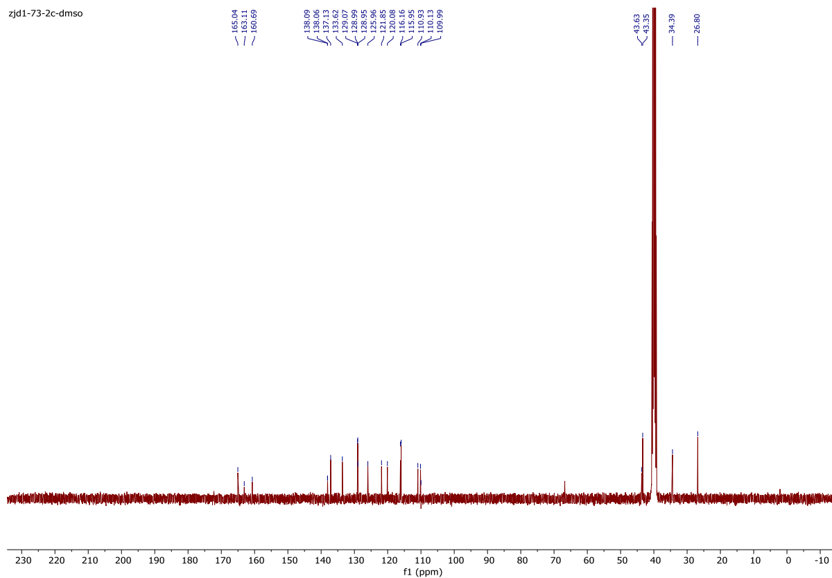
21. 6-(2-Fluorophenyl)-N-(piperidin-4-ylmethyl)-1H-indole-3-carboxamide Hydrochloride (21).
