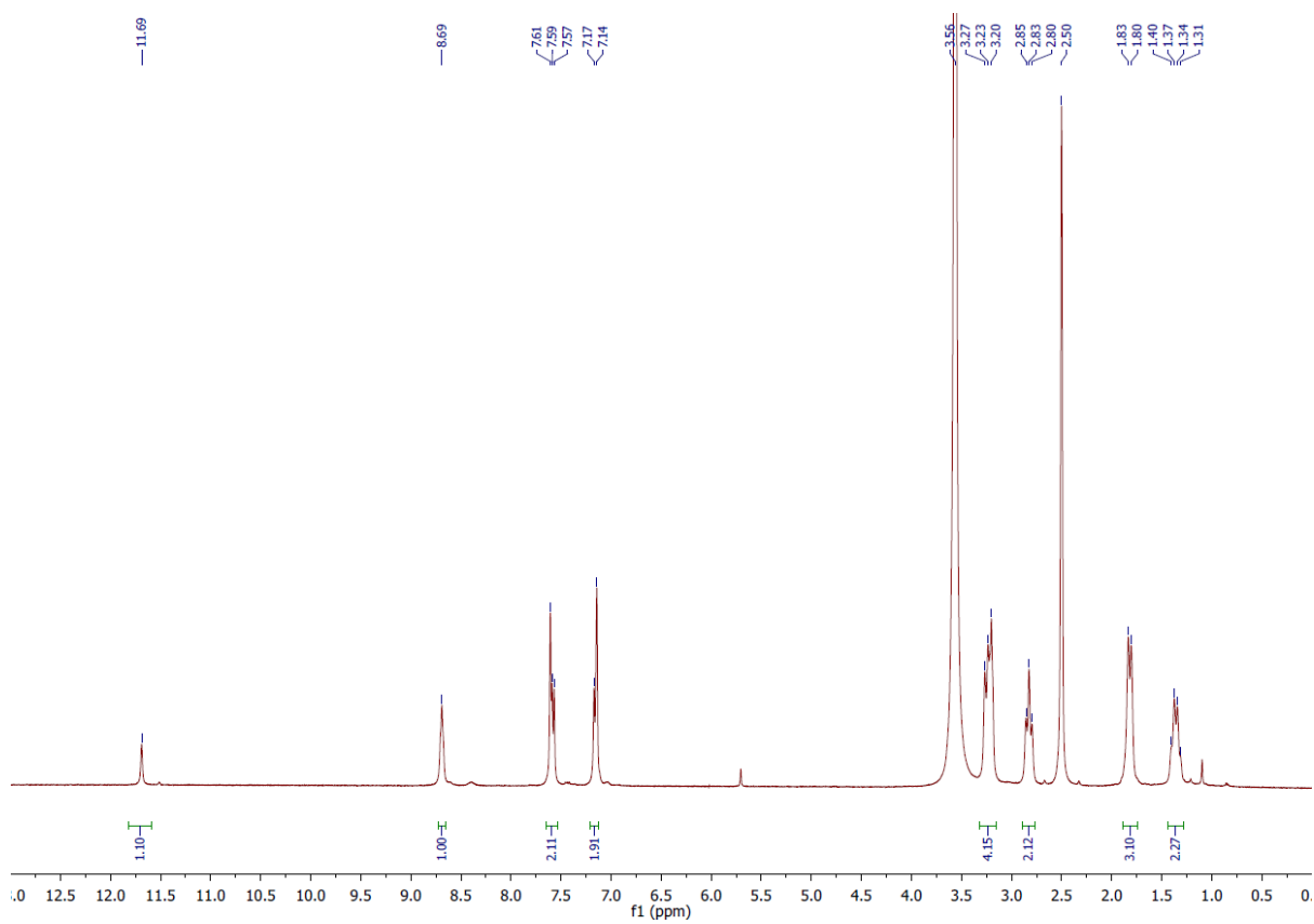
47. N-(Piperidin-4-ylmethyl)-1H-indole-2-carboxamide Hydrochloride (47).
