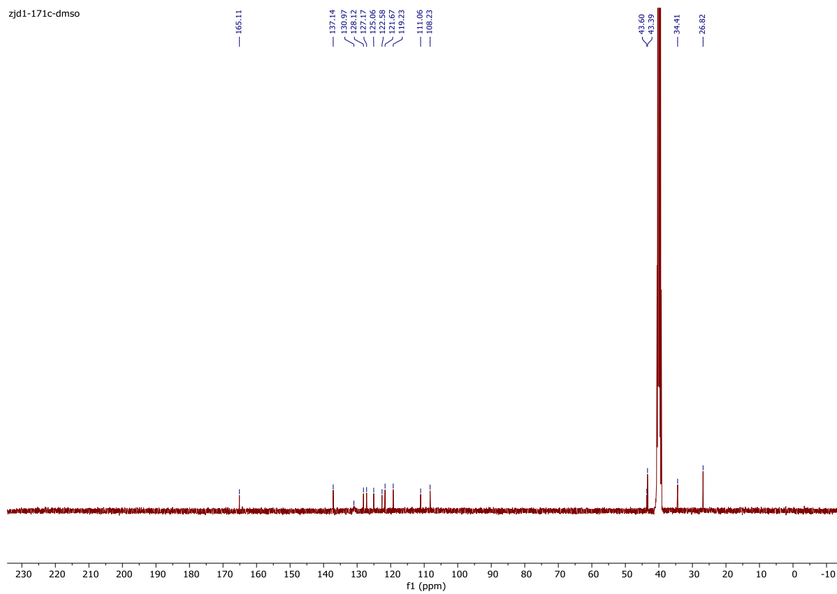
33. N-(Piperidin-4-ylmethyl)-5-(pyridin-3-yl)-1H-indole-2-carboxamide Hydrochloride ( 33 ).
