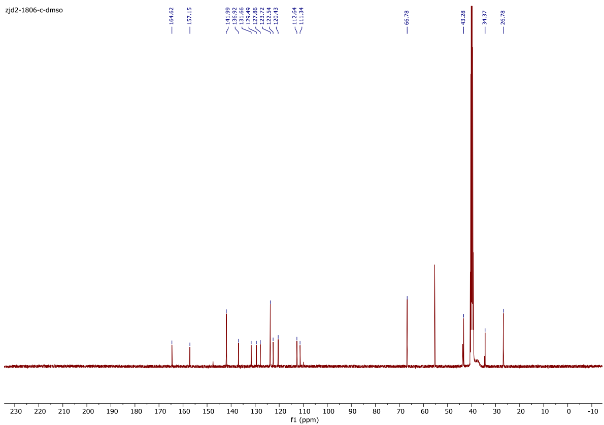
30. N-(Piperidin-4-yl)-6-(pyridin-4-yl)-1H-indole-3-carboxamide Hydrochloride (30).
