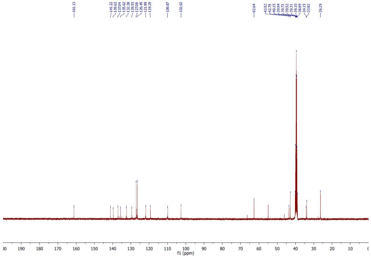
55. 6-(4-(2-Hydroxyethyl)phenyl)-N-(piperidin-4-ylmethyl)-1H-indole-2-carboxamide Hydrochloride ( 55 ).
