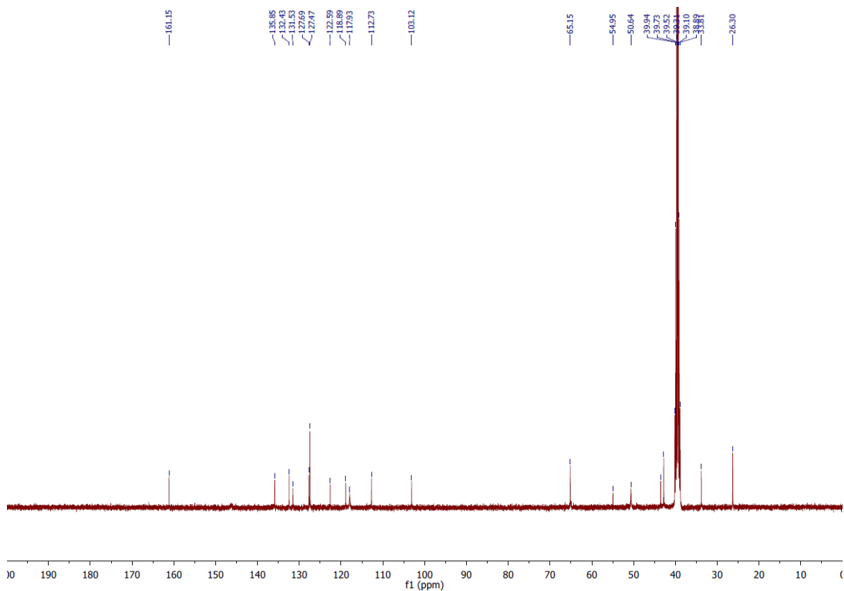
43. 5-(4-(Piperazin-1-yl)phenyl)-N-(piperidin-4-ylmethyl)-1H-indole-2-carboxamide Hydrochloride ( 43 ).
