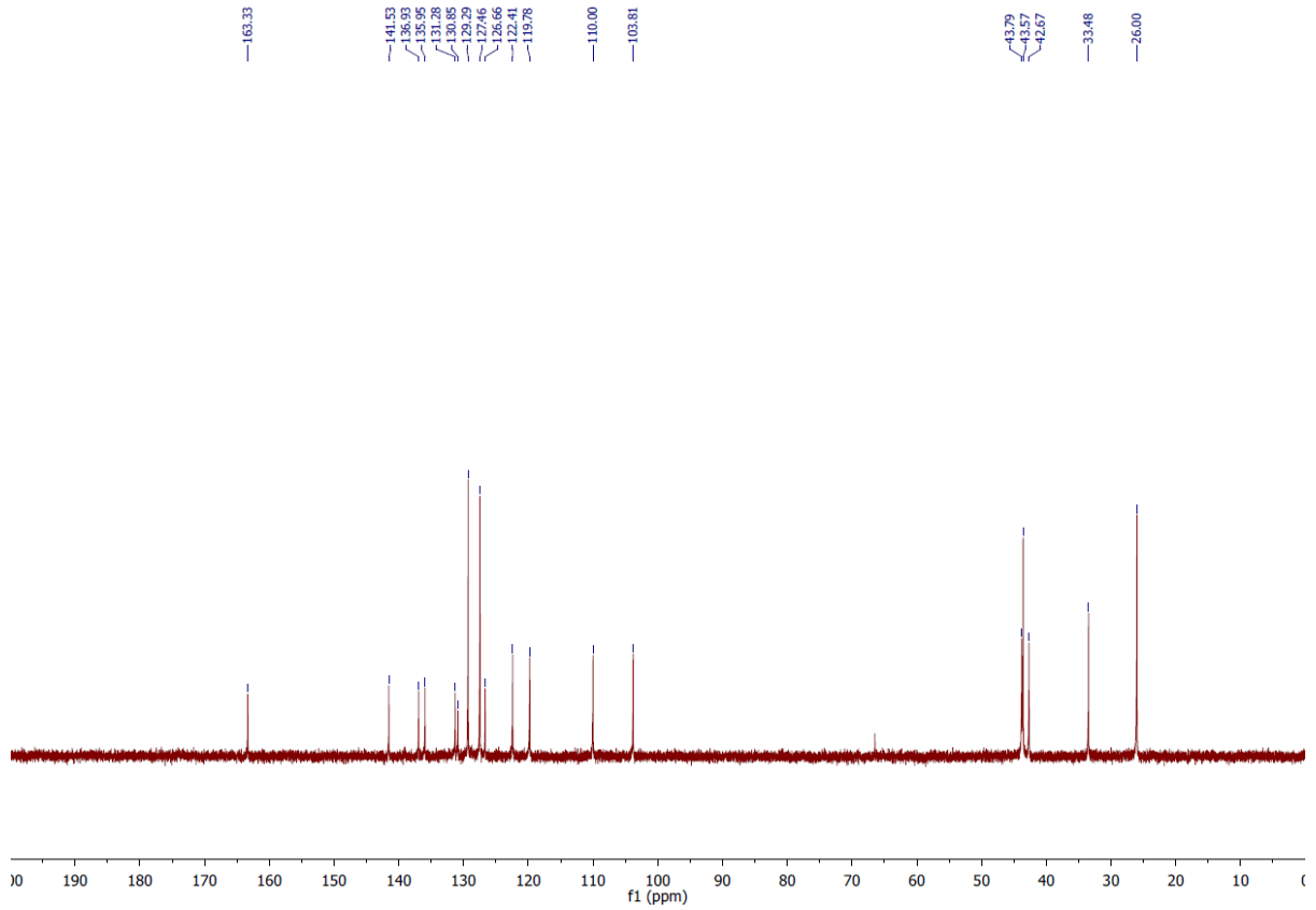
53. 6-(4-Carbamoylphenyl)-N-(piperidin-4-ylmethyl)-1H-indole-2-carboxamide Hydrochloride ( 53 ).
