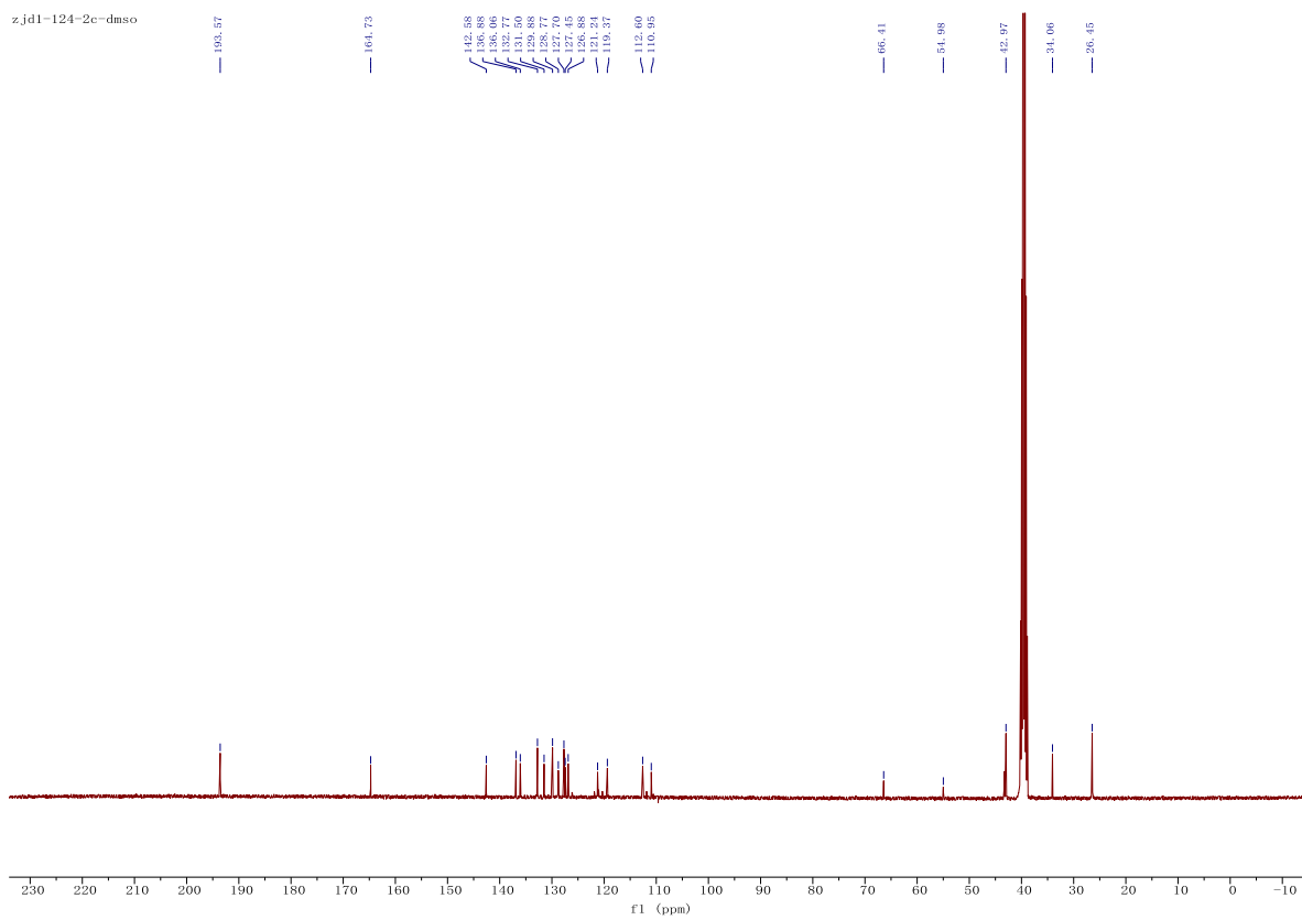
19. N-(Piperidin-4-ylmethyl)-6-(3,4,5-trimethoxyphenyl)-1H-indole-3-carboxamide Hydrochloride (19).
