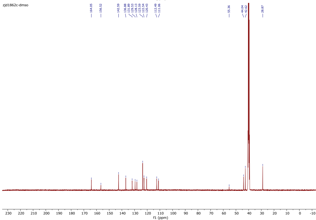
31. N-(2-(Piperidin-4-yl)ethyl)-6-(pyridin-4-yl)-1H-indole-3-carboxamide Hydrochloride (31).
