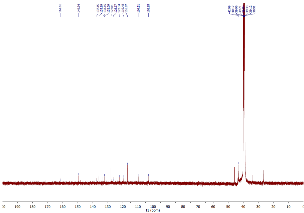
58. 6-(4-(Piperidin-1-yl)phenyl)-N-(piperidin-4-ylmethyl)-1H-indole-2-carboxamide
