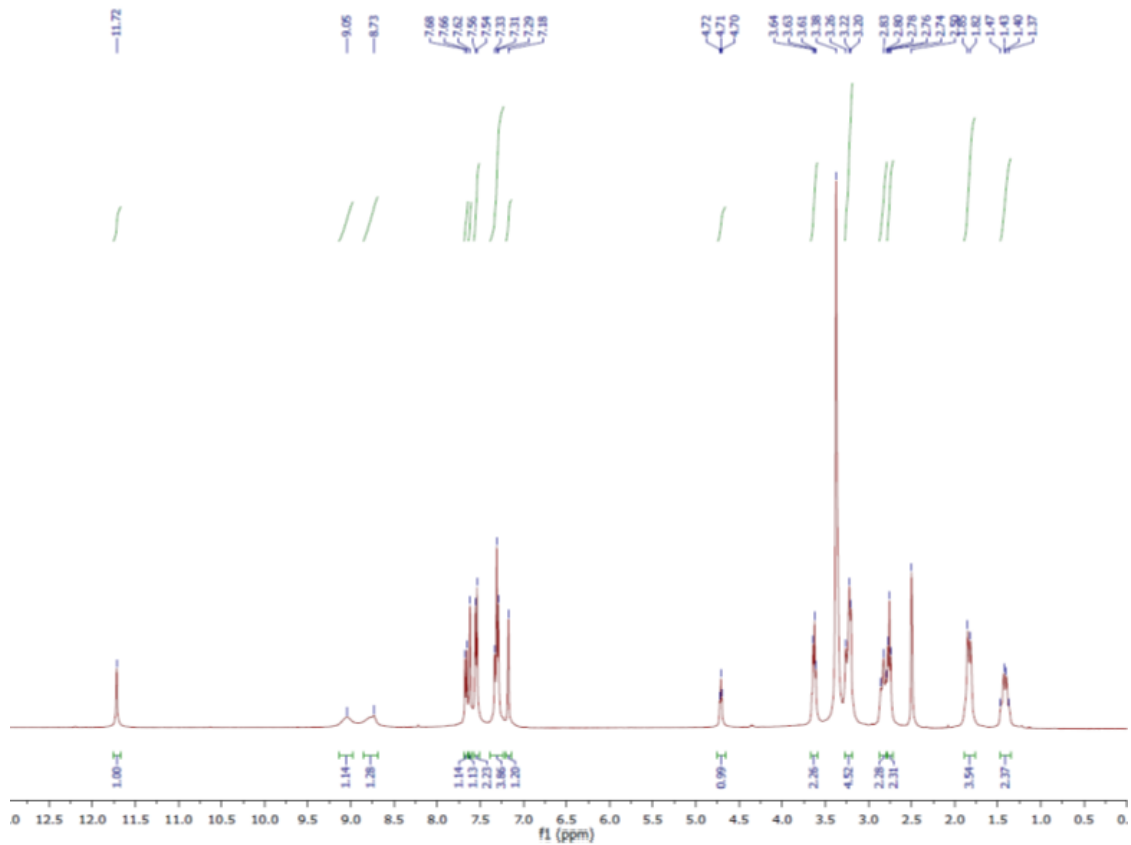
55. 6-(4-(2-Hydroxyethyl)phenyl)-N-(piperidin-4-ylmethyl)-1H-indole-2-carboxamide Hydrochloride ( 55 ).
