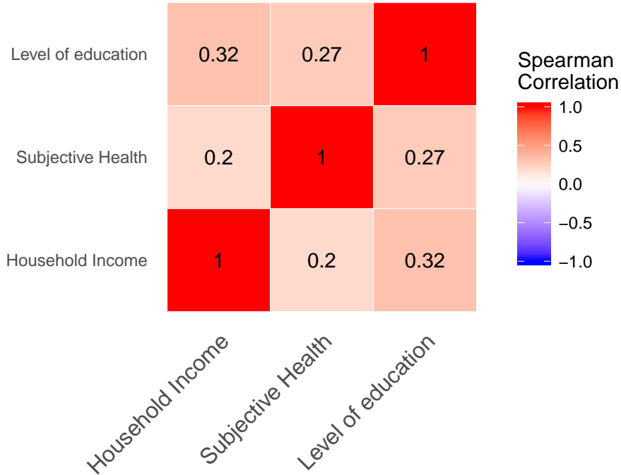
Heatmap of correlation matrix between socioeconomic endpoints in FINRISK
