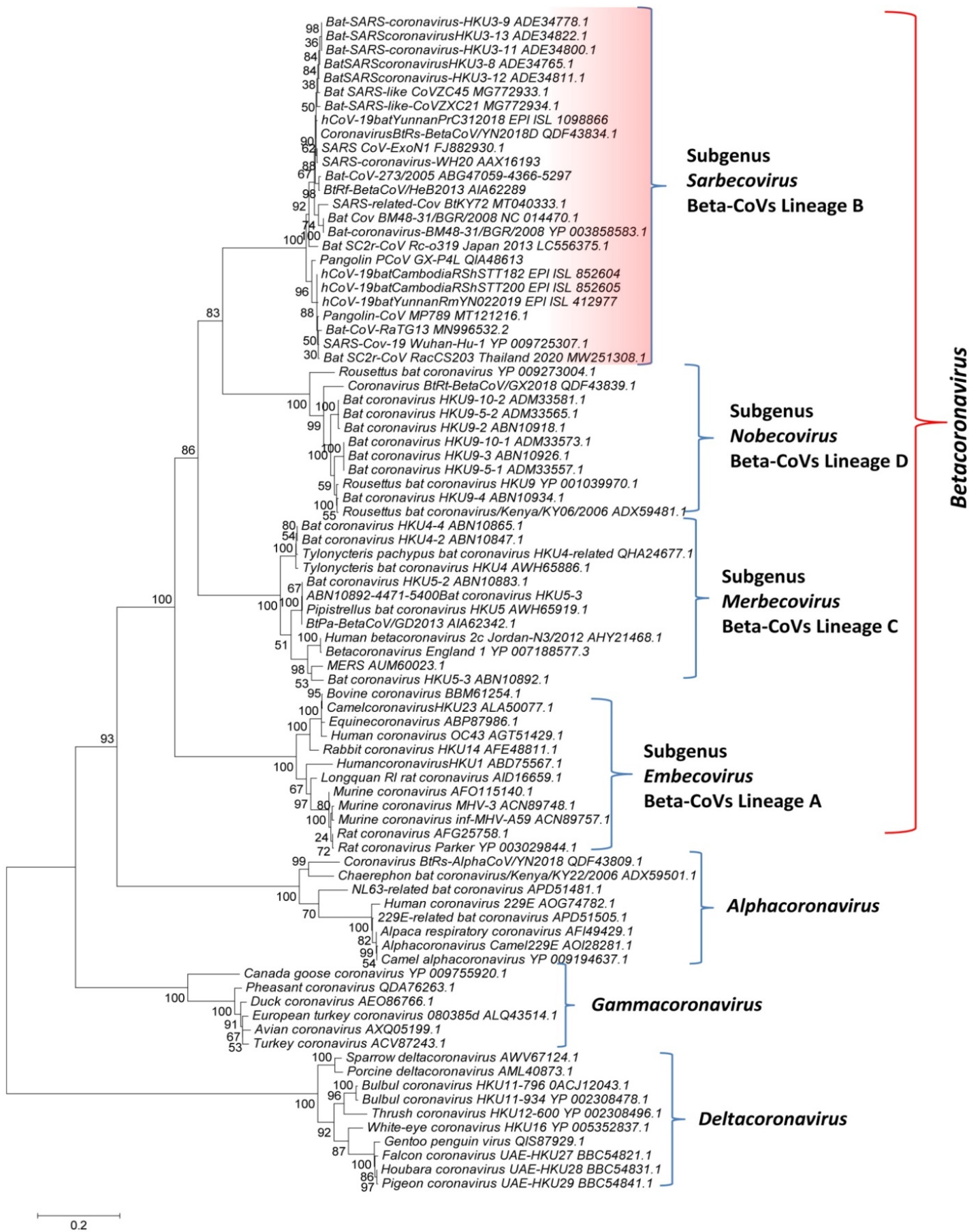
Figure S1. A maximum likelihood tree based on RNA dependent RNA polymerase protein sequences showing the branching of different coronaviruses.
