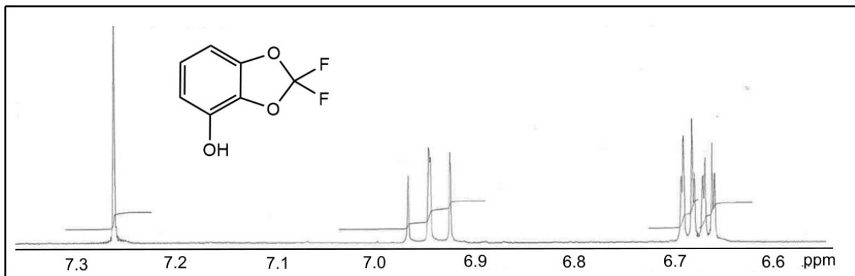
Figure S2. 1 H-NMR in CDCl 3 of the DFBD-4-ol standard
