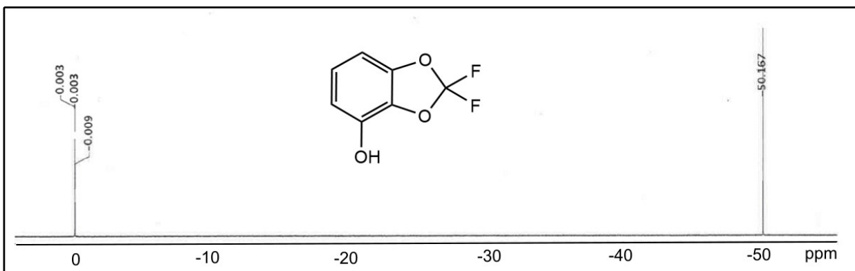
Figure 3S. ^{19}\text{F} -NMR of the DFBD-4-ol standard
