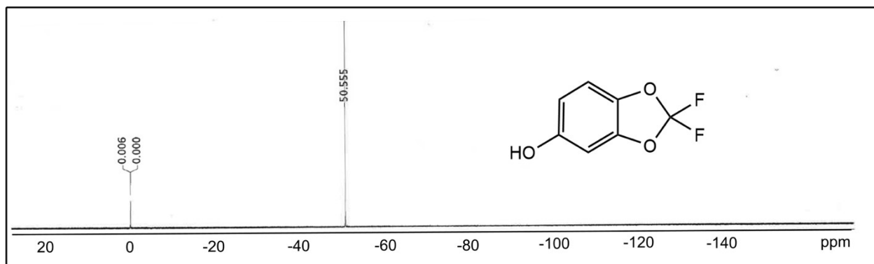
Figure S5. ^{19}\text{F} -NMR of the DFBD-5-ol standard.
