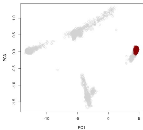
(B) PC1 vs PC3
