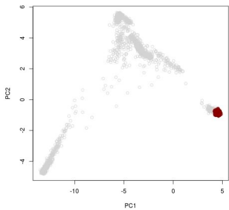
(A) PC1 vs PC2
