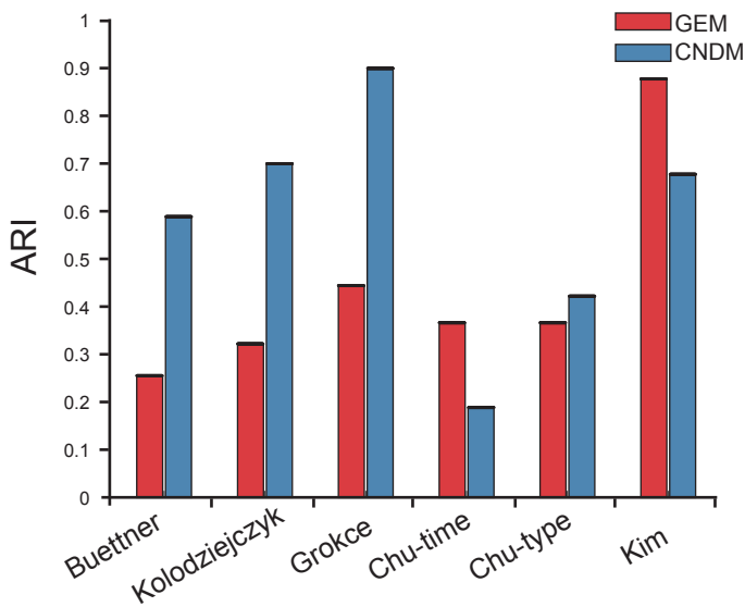
K-medoids
