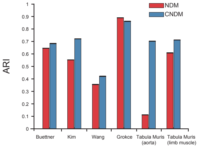
K-medoids
