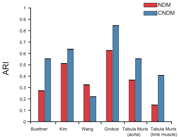
K-medoids
