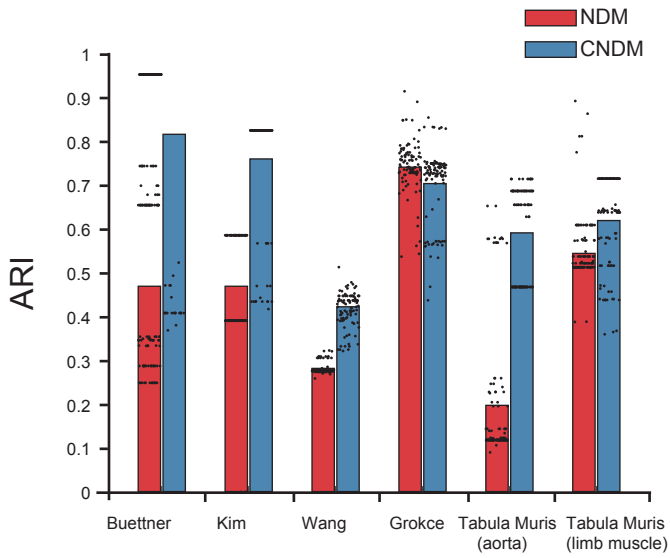
K-means
